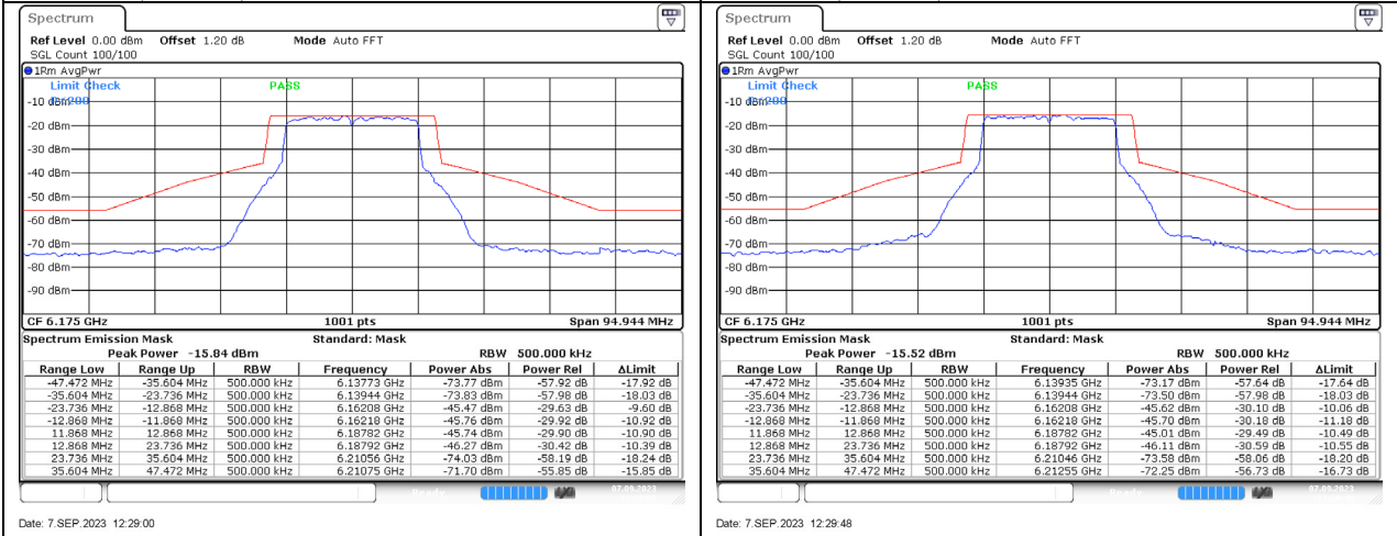
802.11ax (20 MHz) / 6175MHz / Chain A | 802.11ax (20 MHz) / 6175MHz / Chain B
