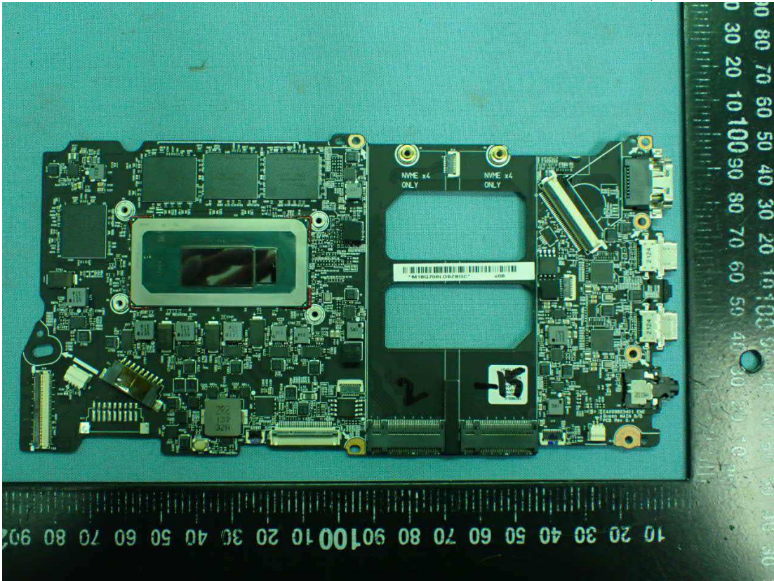
Figure 19 Queen MAIN B/D PCB Main Board, Front View
