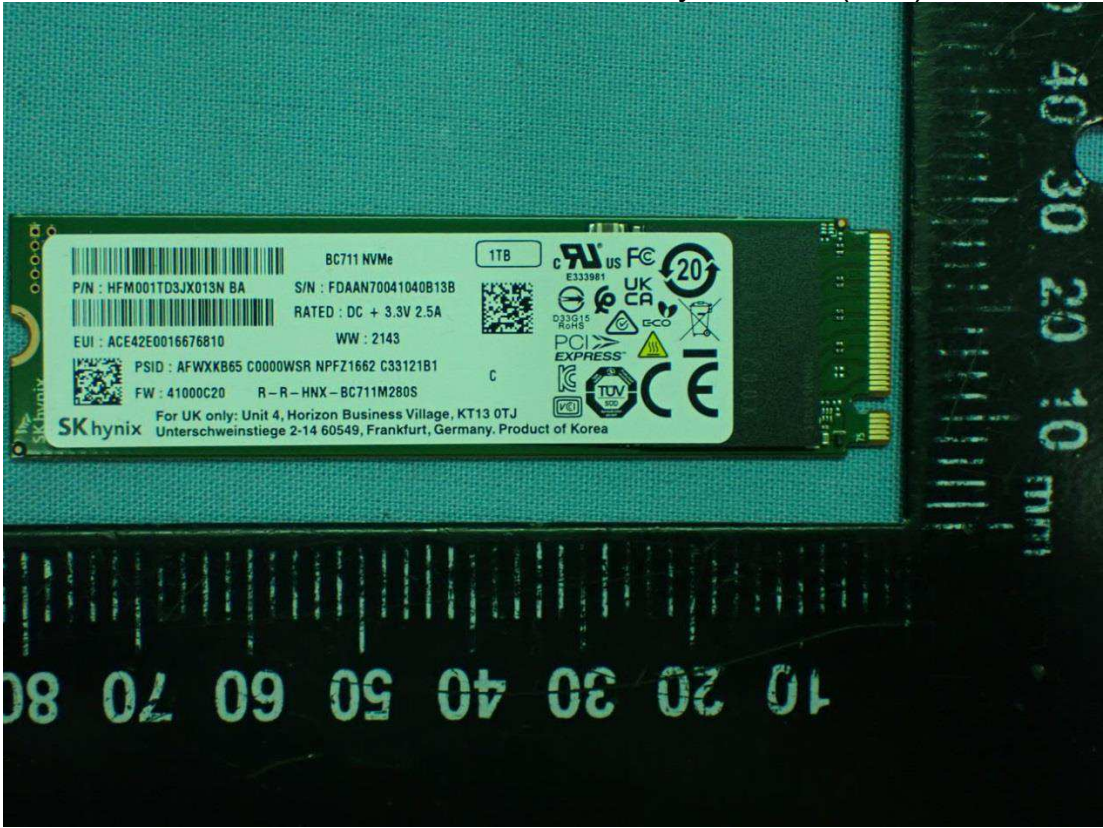
Figure 35 SK hynix, SSD (1TB), Front View
