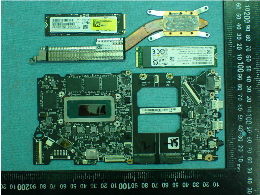
Figure 18 Queen MAIN B/D PCB Main Board, Removed Components
