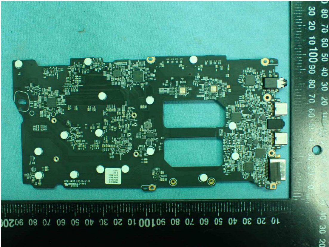
Figure 20 Queen MAIN B/D PCB Main Board, Back View
