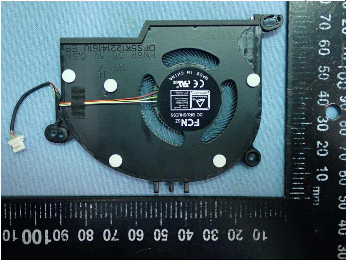
Figure 17 Internal View (DC Fan)
