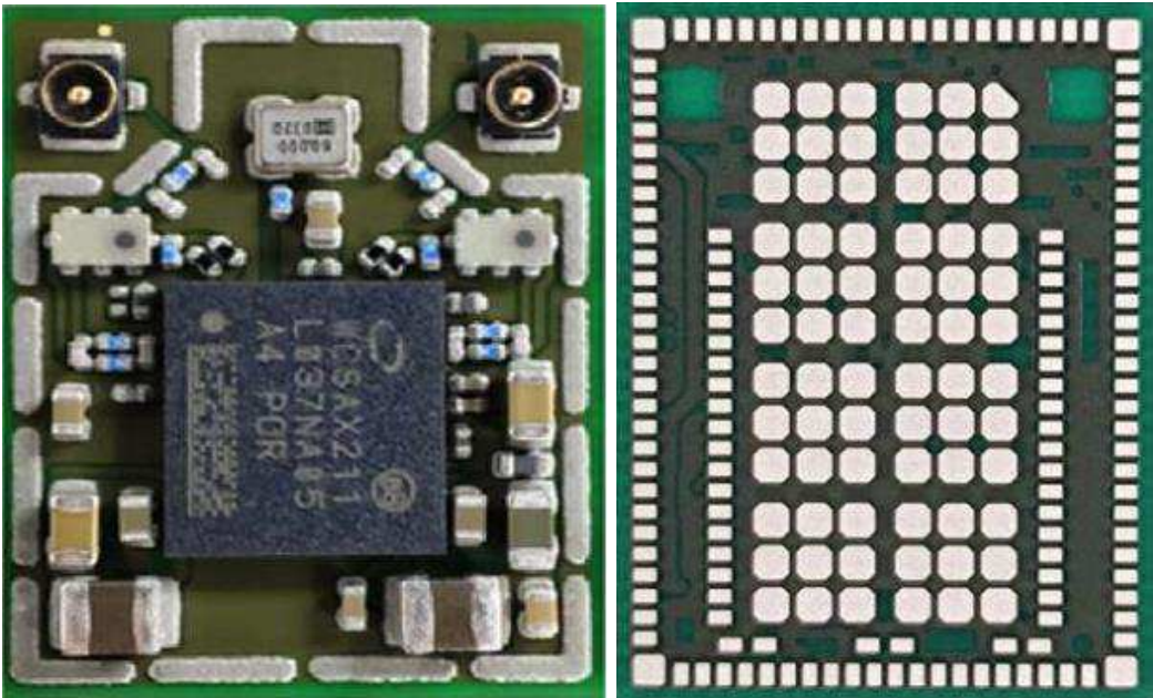
Figure 25 WLAN Combo Card, Without Shield and Back View
