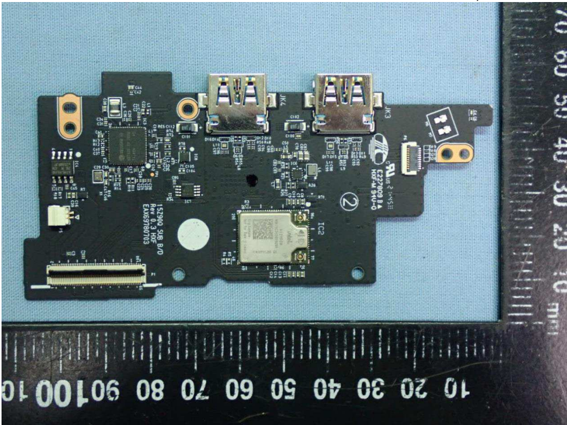
Figure 22 WLAN SUB Board, Front View
