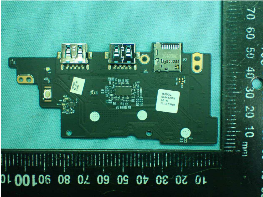
Figure 23 WLAN SUB Board, Back View
