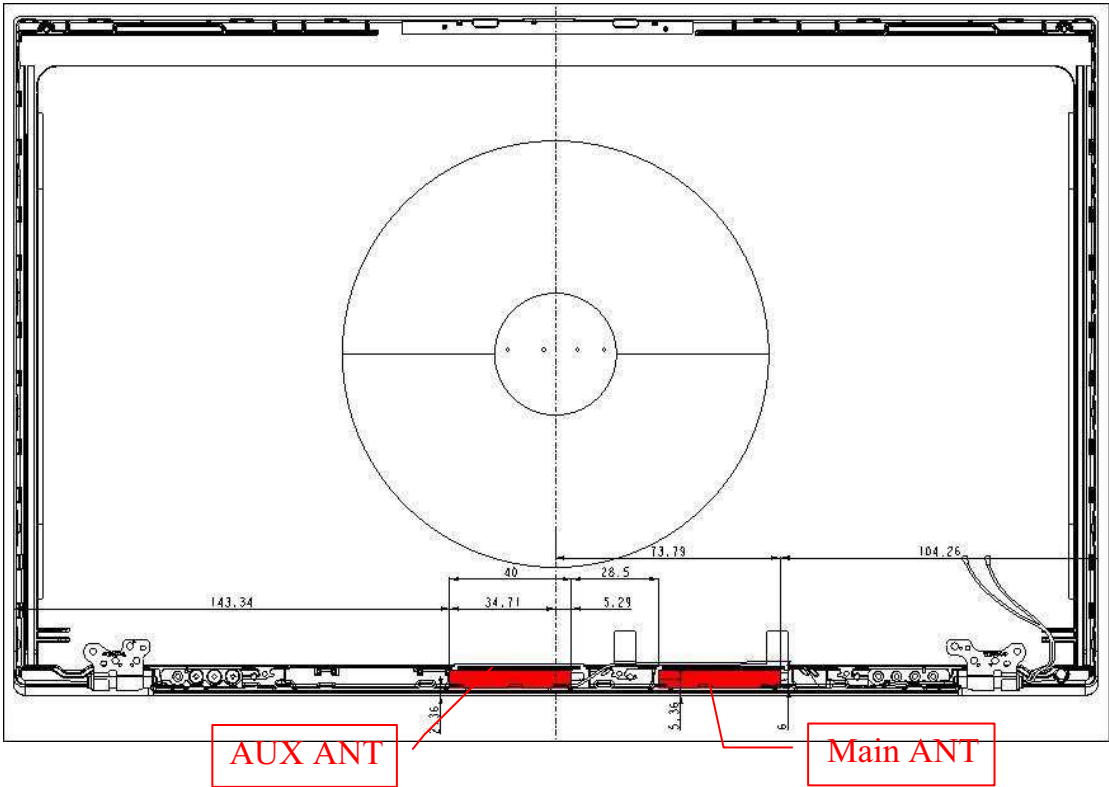
Figure 32 WLAN Combo Antenna Position
