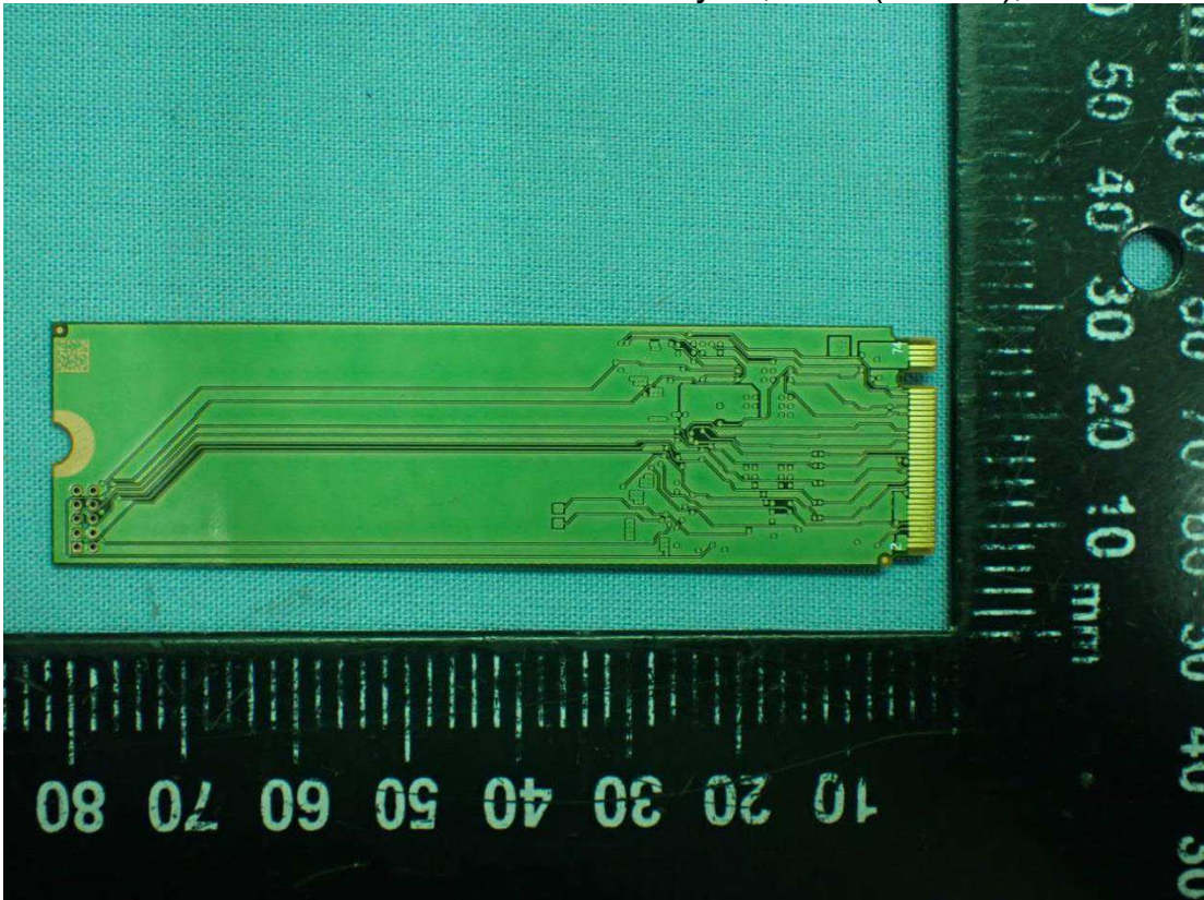
Figure 40 SK hynix, SSD (256GB), Back View
