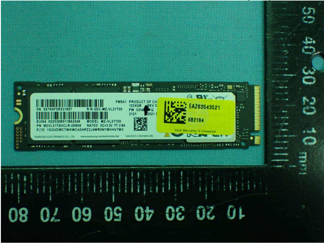
Figure 37 SAMSUNG, SSD (1TB), Front View
