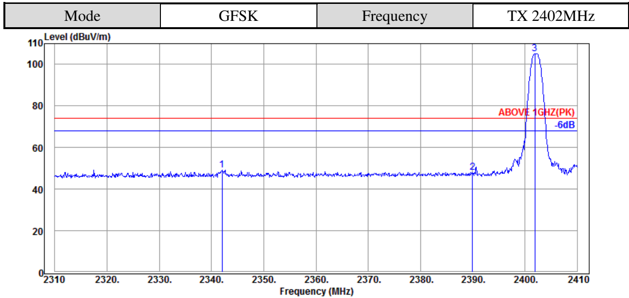
Antenna at Vertical Polarization
