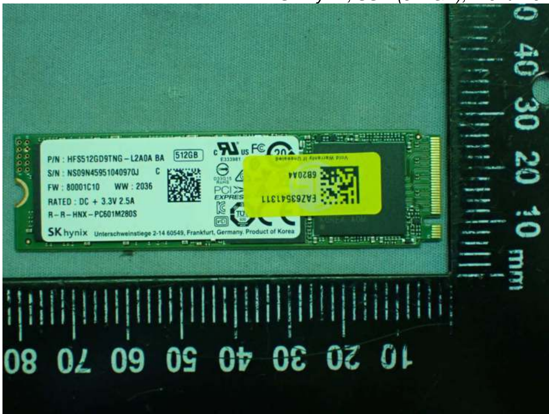
Figure 43 SK hynix, SSD (512GB), Front View
