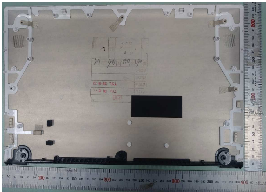
Figure 16 Internal View
