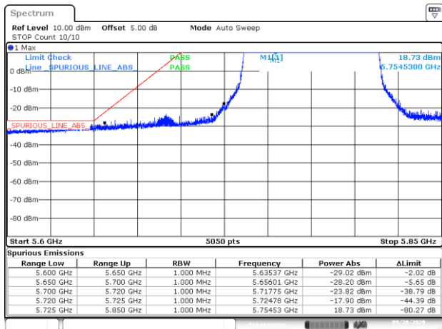
BE-NR-LOW, SISO-B, 802.11ac80-HE0, Ch155
