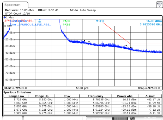
BE-NR-HIGH, SISO-B, 802.11ac80-VHT0, Ch155
