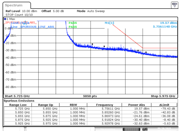
BE-NR-HIGH, SISO-B, 802.11ac80-HE0, Ch155
