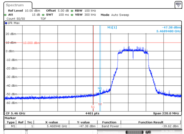
BE-NR-LOW, MIMO-B, 802.11ax40-HE0, Ch102
