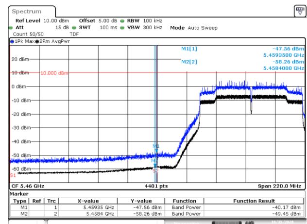
BE-R-LOW, MIMO-A, 802.11ac80-VHT0, Ch106
