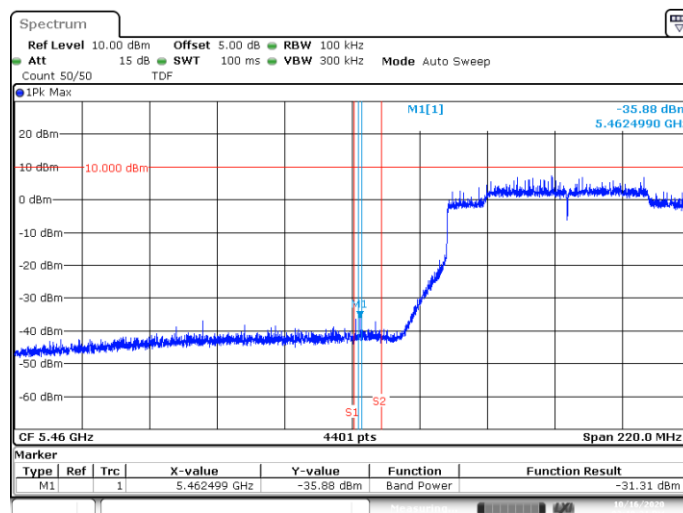
BE-NR-LOW, SISO-B, 802.11ax80-HE0, Ch106
