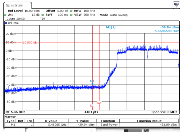
BE-NR-LOW, SISO-B, 802.11ac80-VHT0, Ch106
