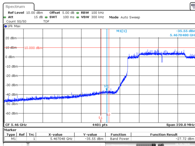
BE-NR-LOW, SISO-A, 802.11ax80-HE0, Ch106
