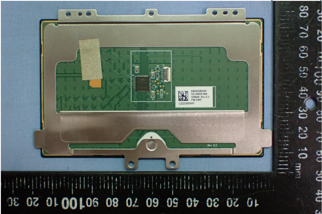
Figure 31 Touch Pad (Back View)
