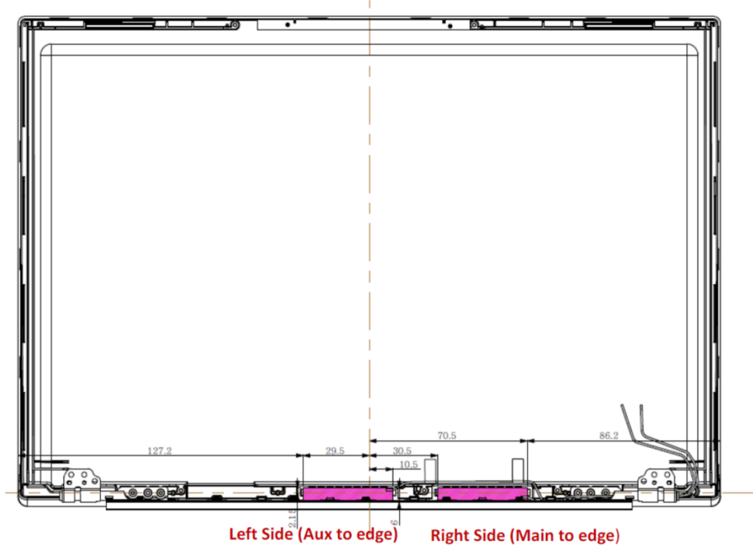
Figure 36 WA-P-LELE-04-025, WLAN Combo Antenna Position
