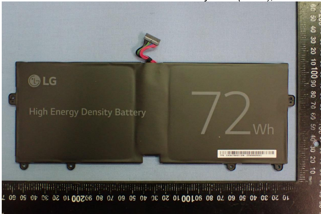
Figure 23 Battery Pack (72Wh), Front View
