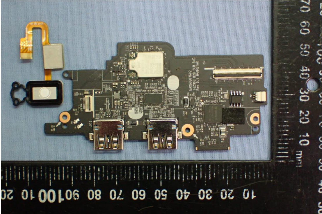
Figure 16 Internal View
