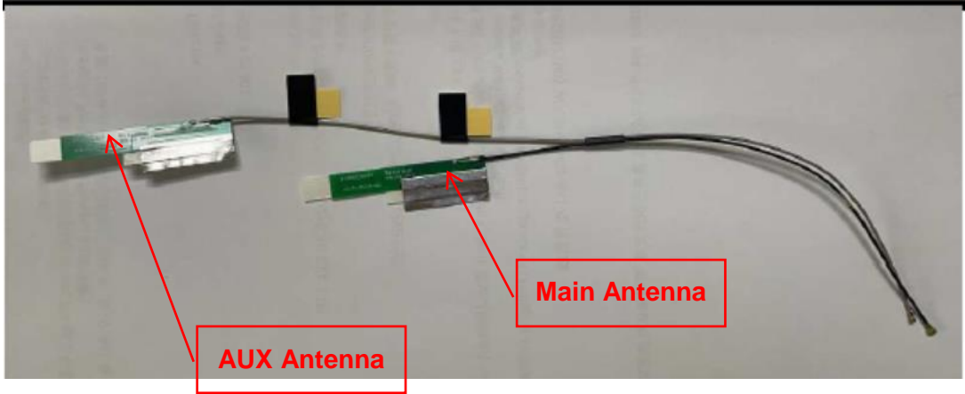
Figure 34 WA-P-LELE-04-025, WLAN Combo Antenna
