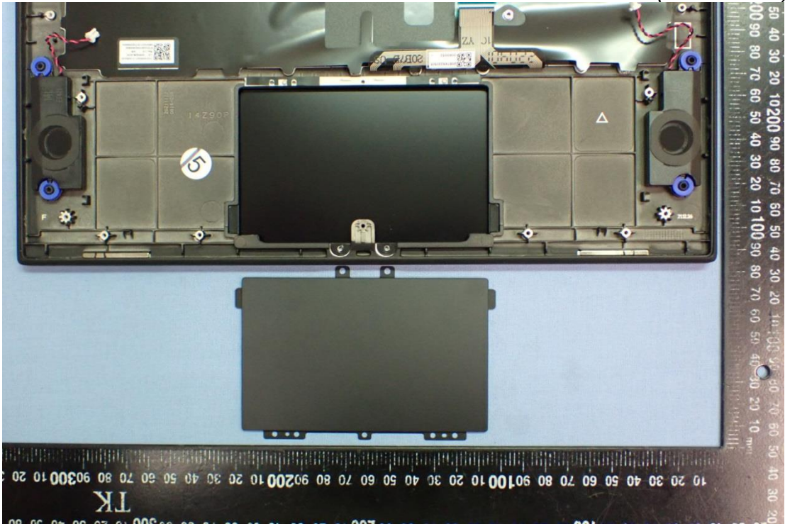
Figure 30 Touch Pad (Front View)
