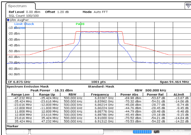
802.11ax-20 MHz / 6875 MHz / Chain A
