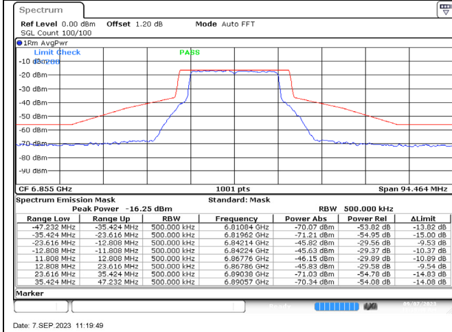
802.11ax-20 MHz / 6855 MHz / Chain A
