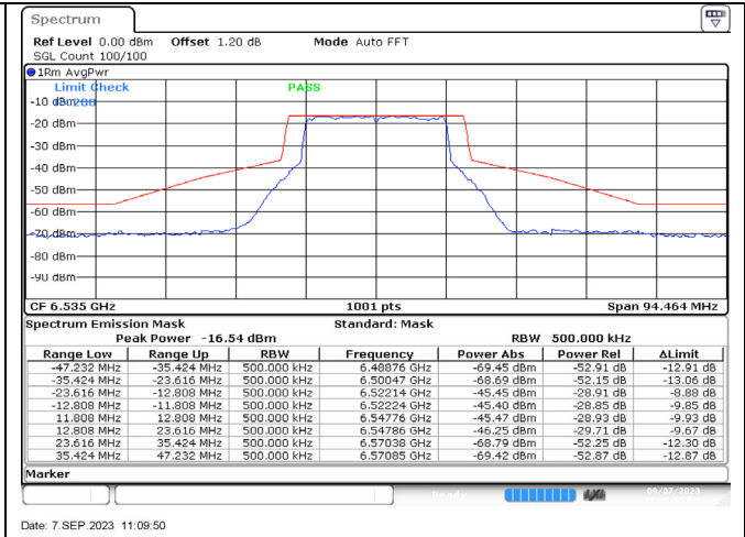
802.11ax-20 MHz / 6535 MHz / Chain B
