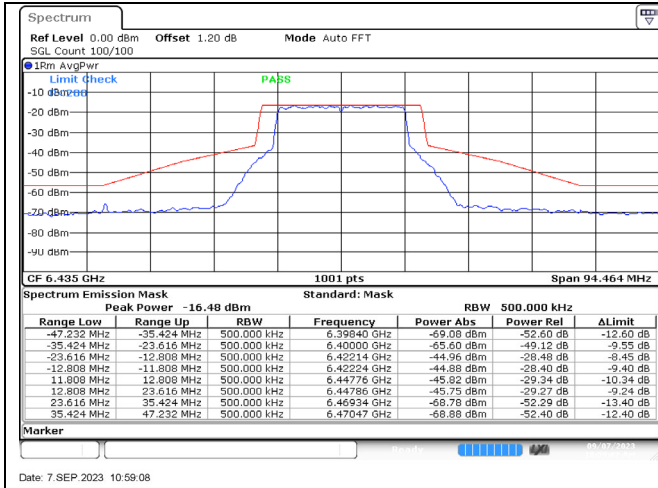
802.11ax-20 MHz / 6435 MHz / Chain A
