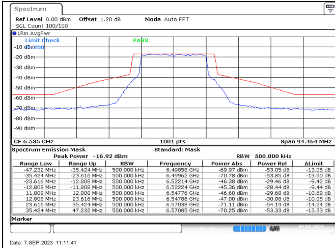
802.11ax-20 MHz / 6535 MHz / Chain A
