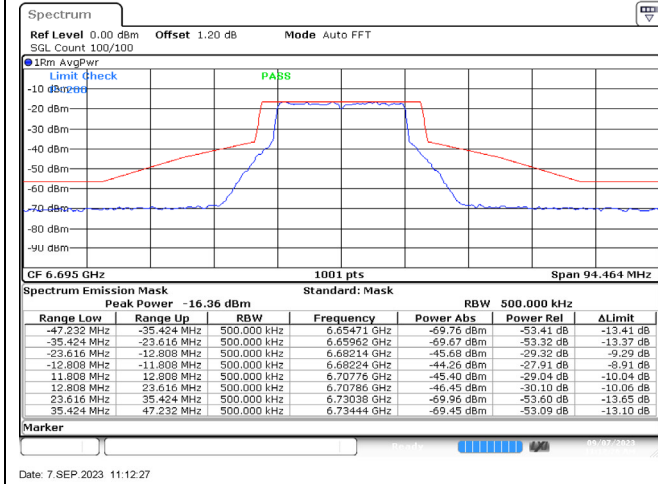
802.11ax-20 MHz / 6695 MHz / Chain A
