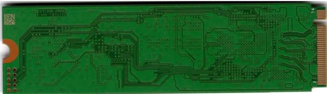
Figure 42 SSD, SK hynix, (512GB), Back View
