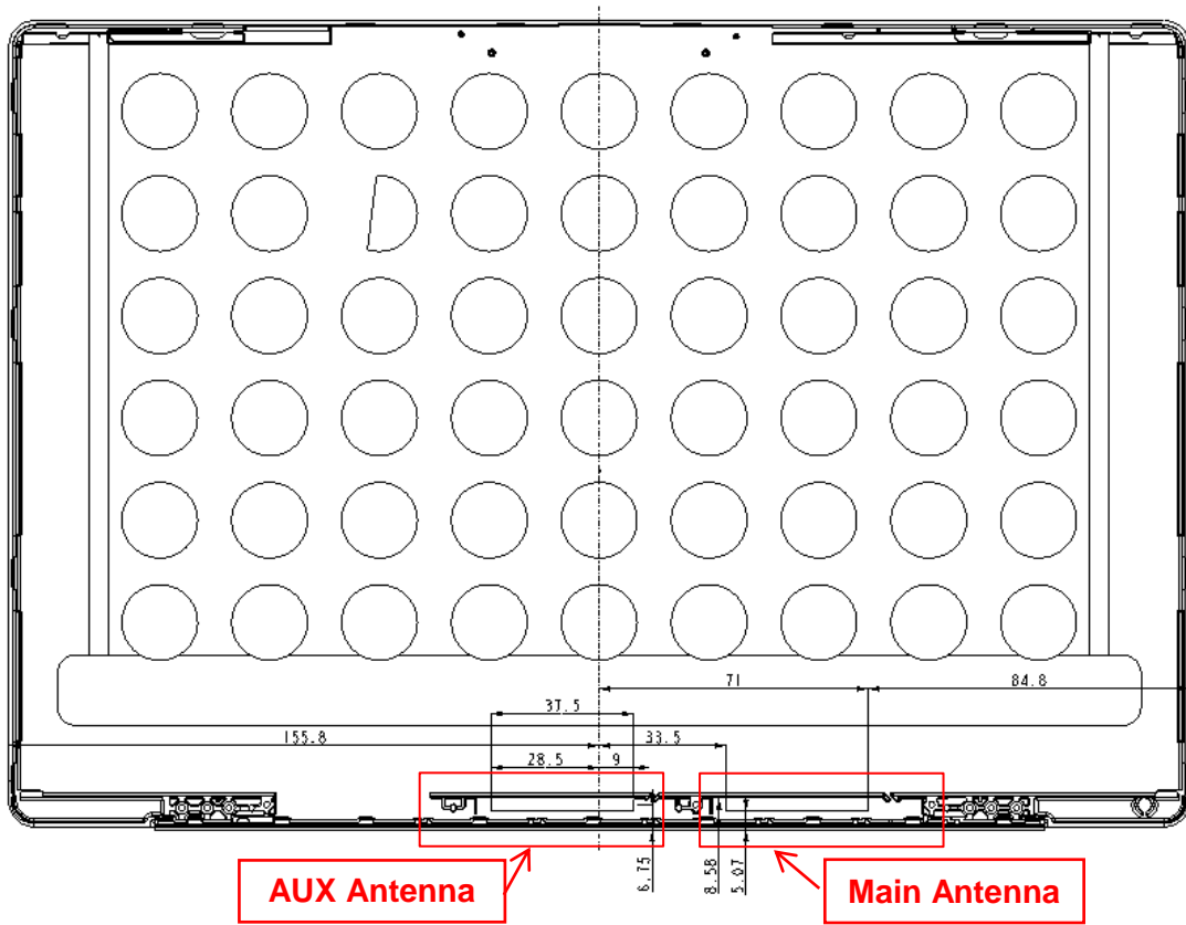
Figure 55 WLAN Combo Antenna Position
