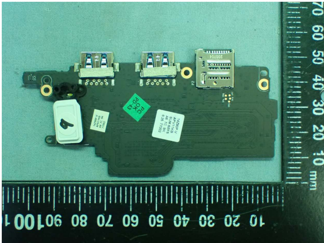
Figure 42 WLAN SUB Board, Back View
