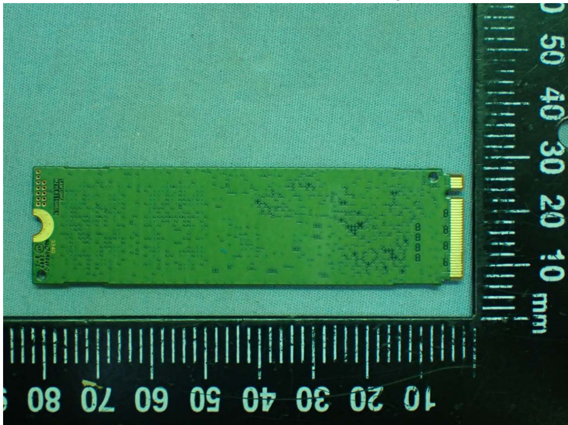
Figure 44 Samsung, 1TB, SSD, Back View
