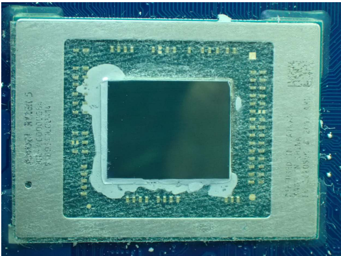
Figure 56 i5-1135G7, CPU View
