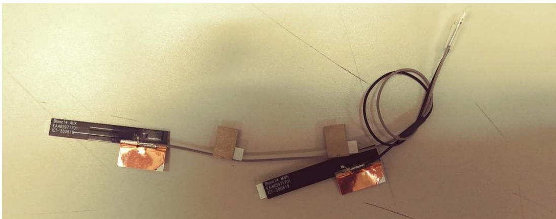
Figure 60 LG (LUXSHARE-ICT), WLAN Combo Antenna, Back View
