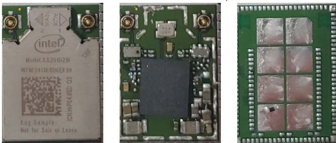
Figure 58 WLAN Combo Card, Remove Cover / Back View
