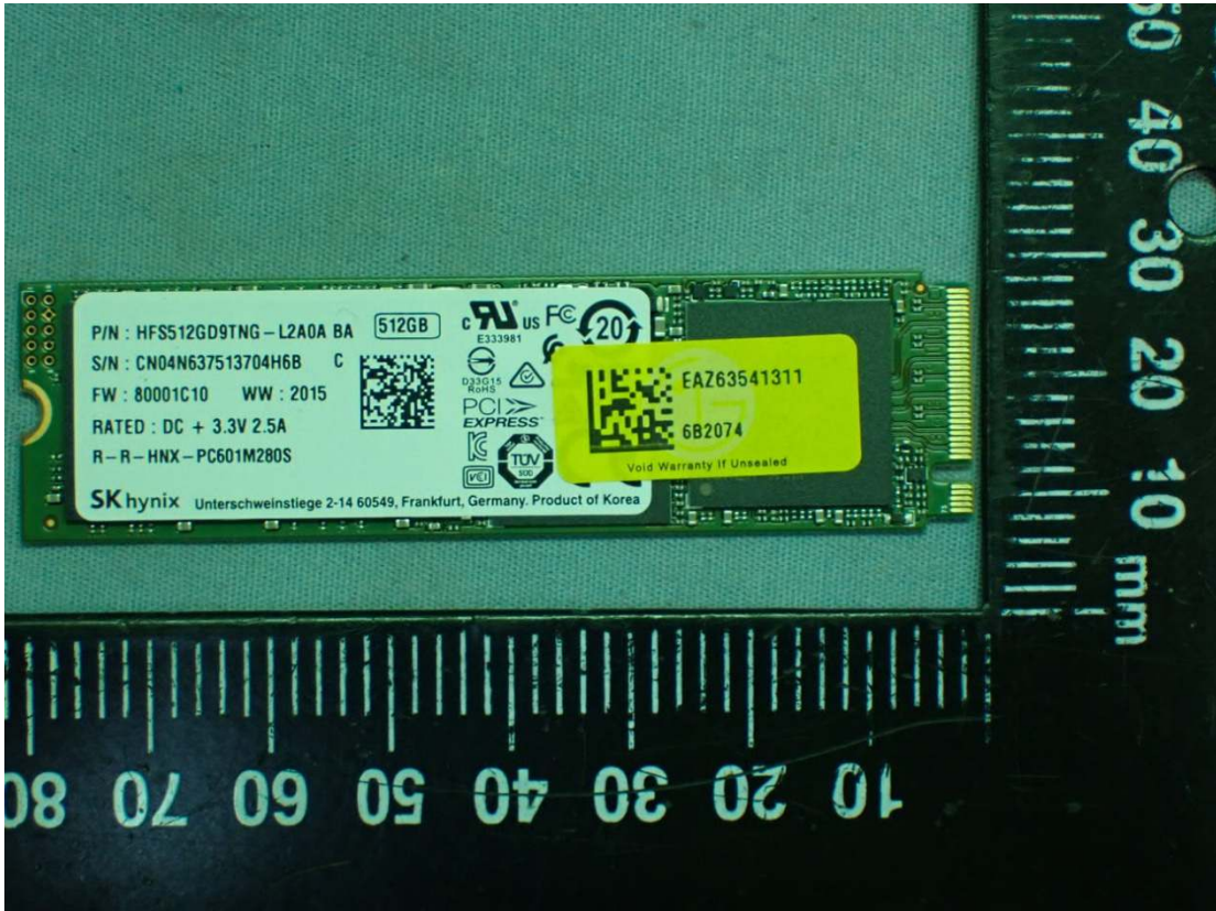
Figure 53 SK hynix, 512GB, SSD, Front View
