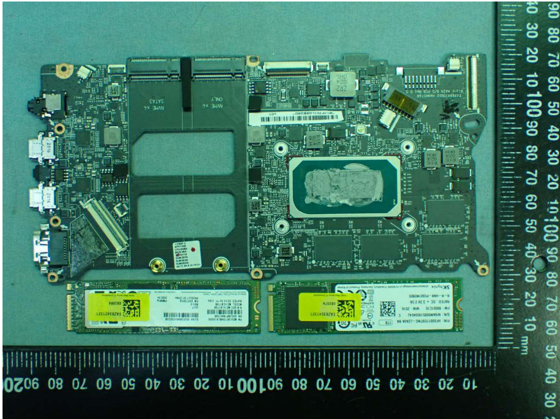
Figure 36 Internal View
