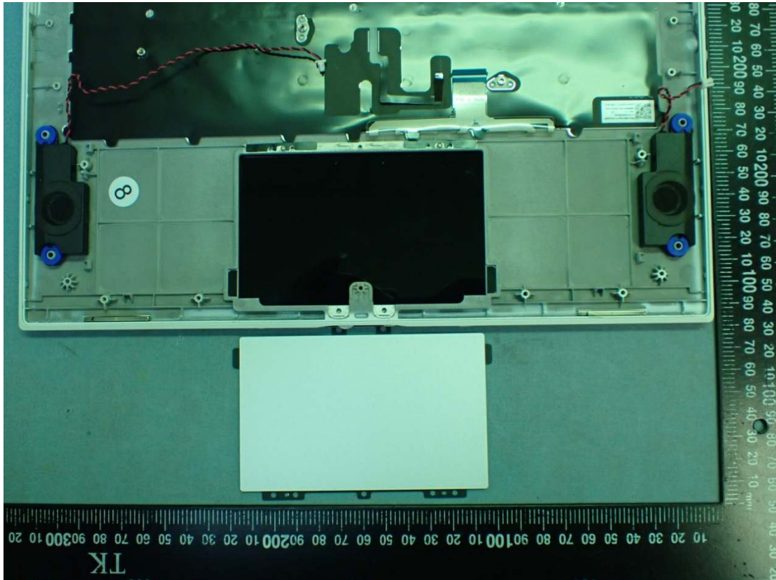
Figure 35 Internal View
