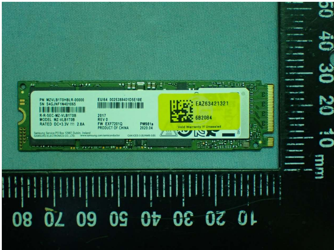
Figure 43 Samsung, 1TB, SSD, Front View
