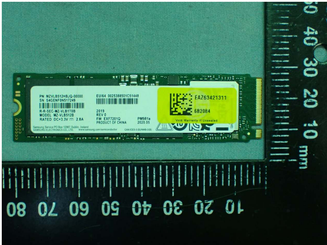
Figure 45 Samsung, 512GB, SSD, Front View
