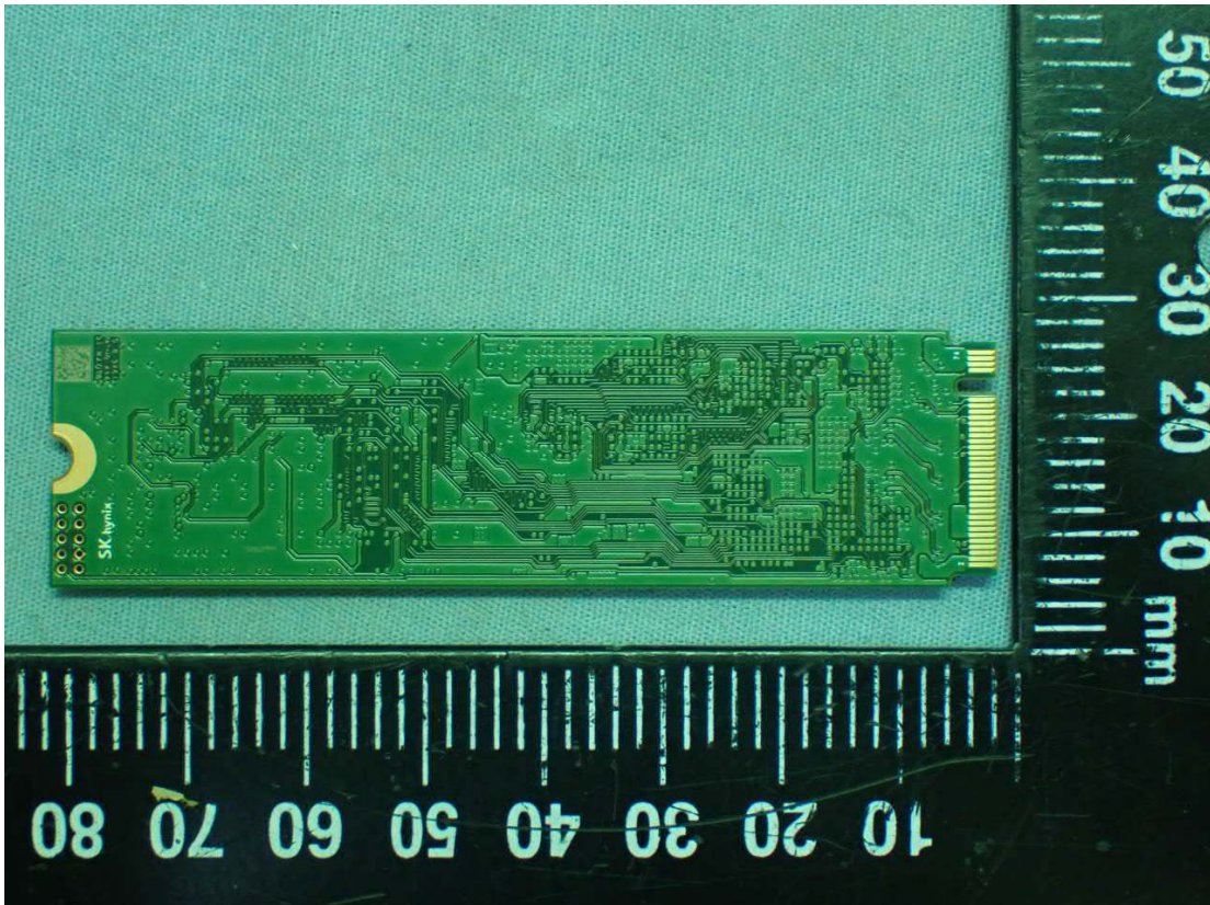
Figure 52 SK hynix, 1TB, SSD, Back View
