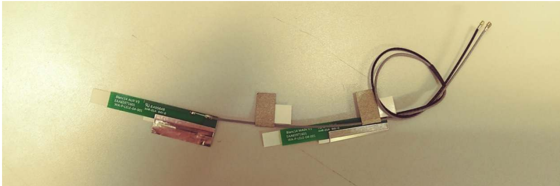
Figure 60 LG (LUXSHARE-ICT), WLAN Combo Antenna, Back View
