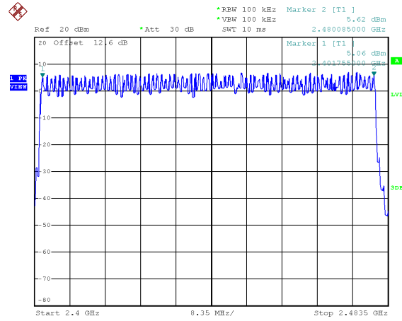
3 Mbps
