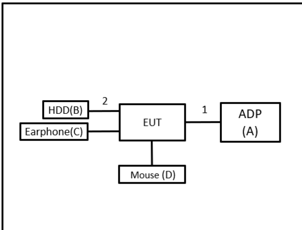
Radiated Emissions
