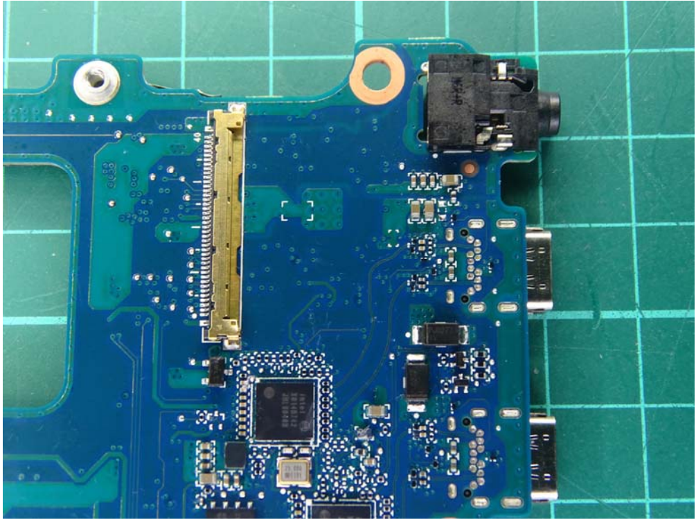
(43) EUT Photo
