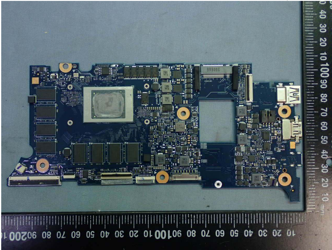
Figure 26 Main Board, Front View
