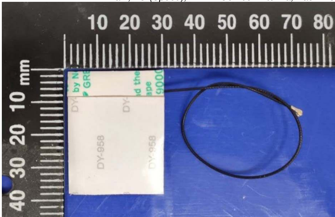
Figure 53 Main, LG (Speed), WLAN Combo Antenna, Back View
