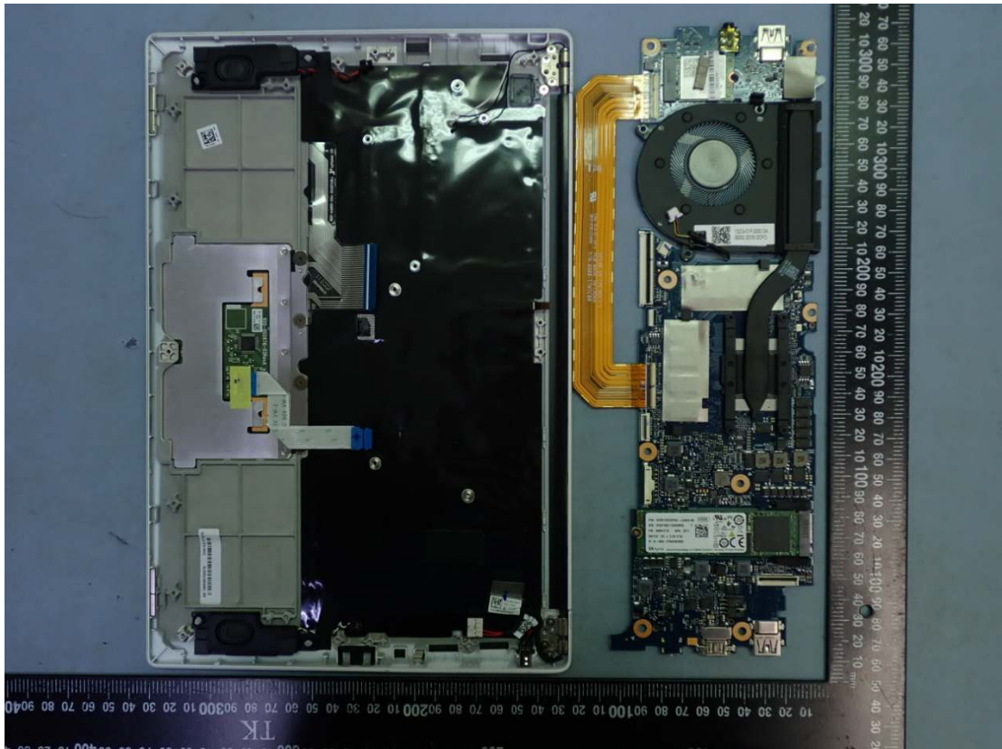
Figure 19 Internal View
