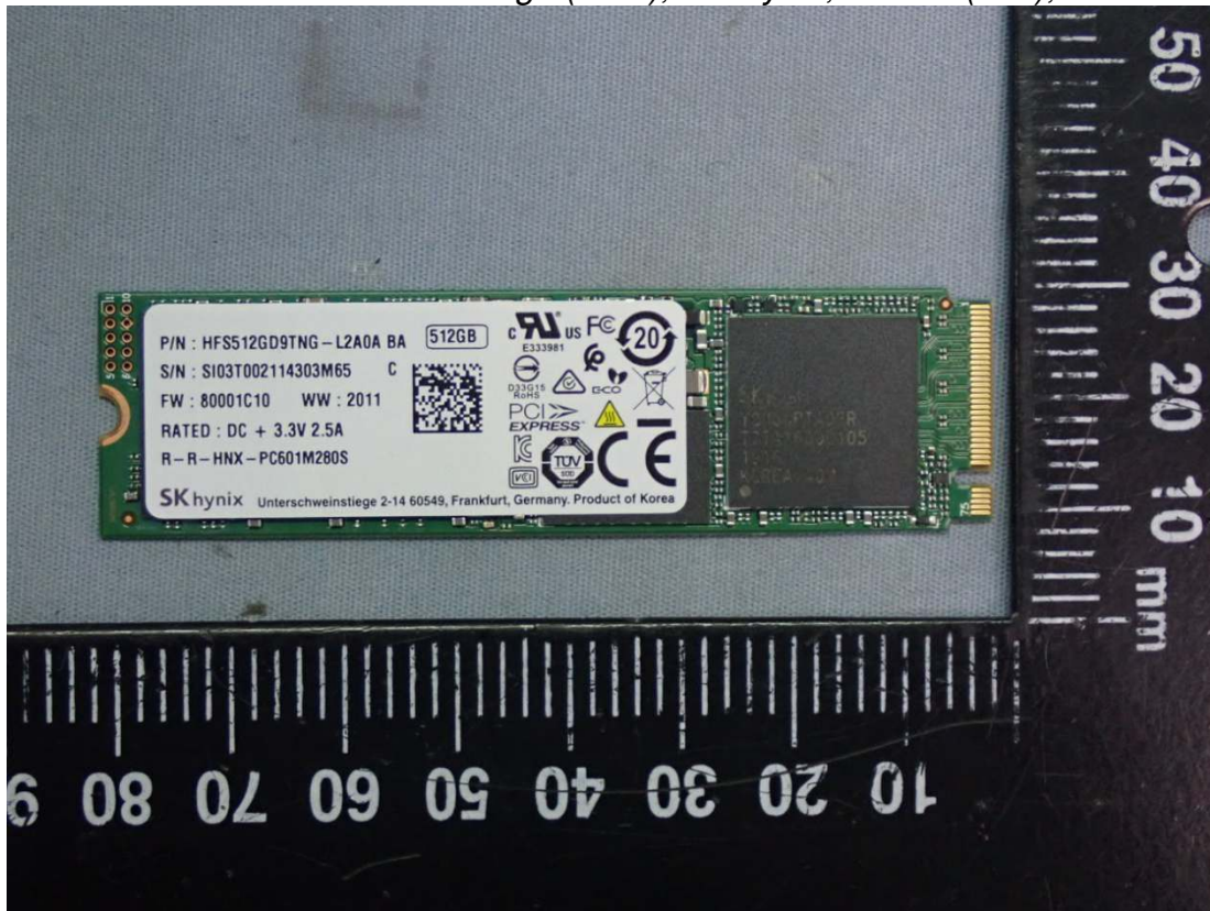
Figure 30 Storage (SSD), SK Hynix, 512GB (M.2), Front View
