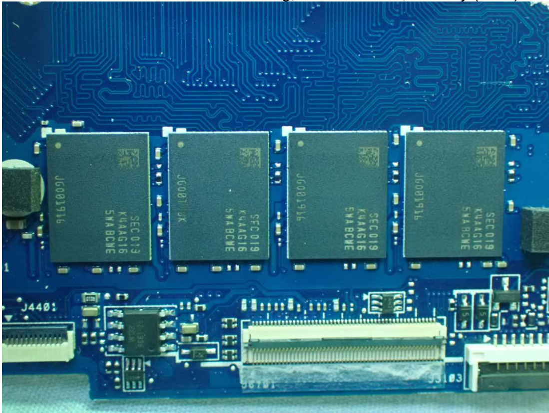
Figure 38 Samsung, 16GB View #1, Memory (RAM) View
