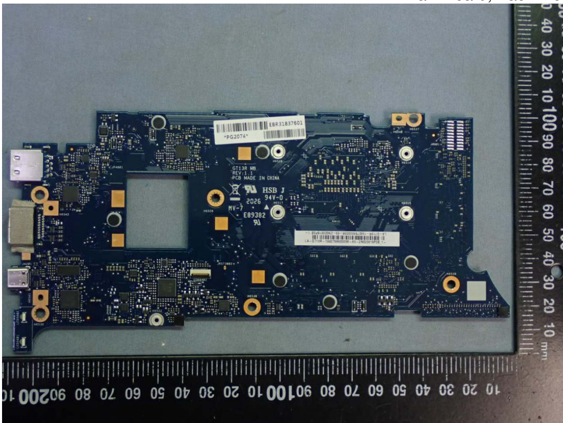
Figure 27 Main Board, Back View
