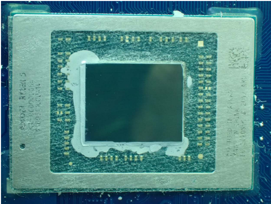
Figure 43 RYZEN 5 4500U, CPU View
