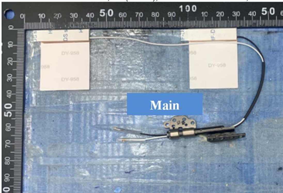
Figure 49 Main, LG (AWAN), WLAN Combo Antenna, Back View
