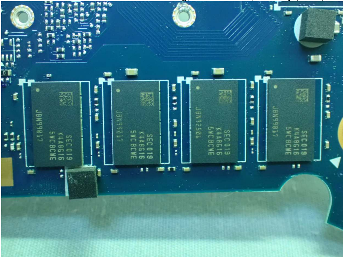
Figure 41 Samsung, 8GB View #2, Memory (RAM) View
