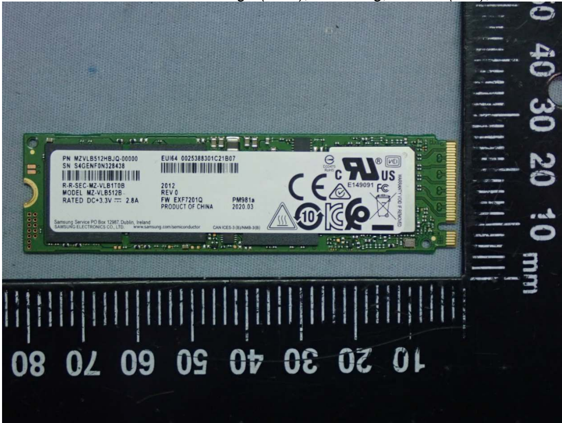
Figure 32 Storage (SSD), Samsung, 512GB (M.2), Front View
