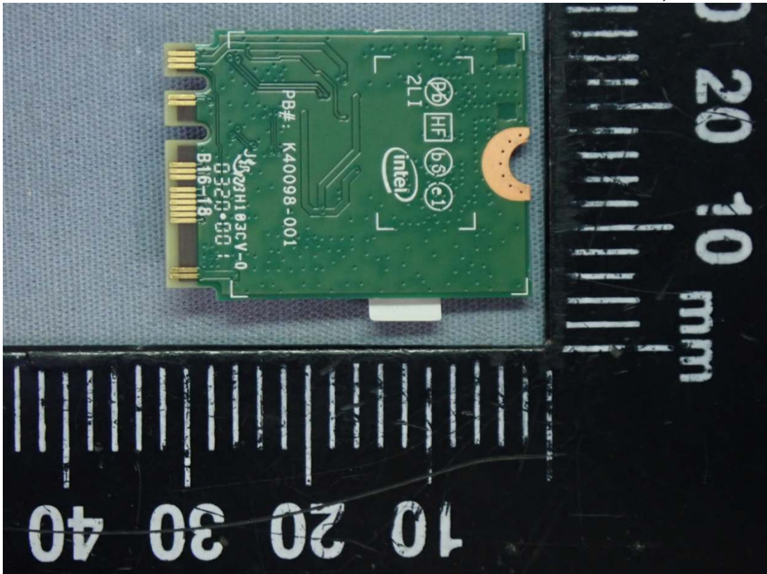
Figure 45 WLAN Combo Card, Front View
