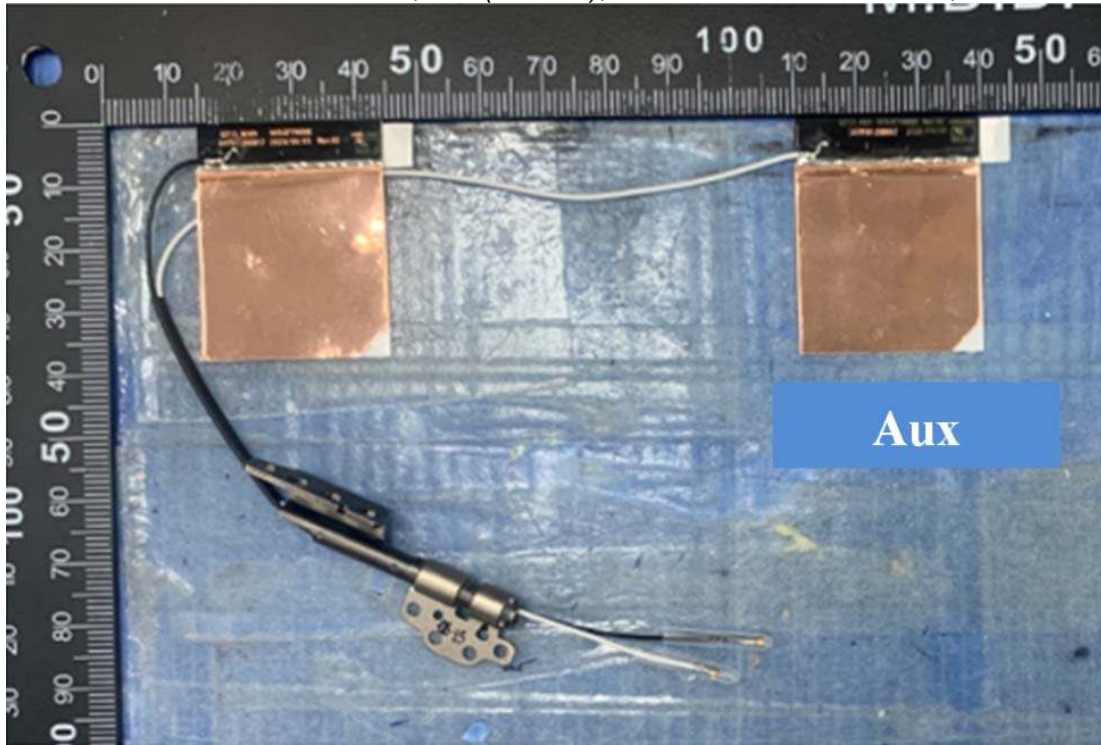
Figure 50 AUX, LG (AWAN), WLAN Combo Antenna, Front View
