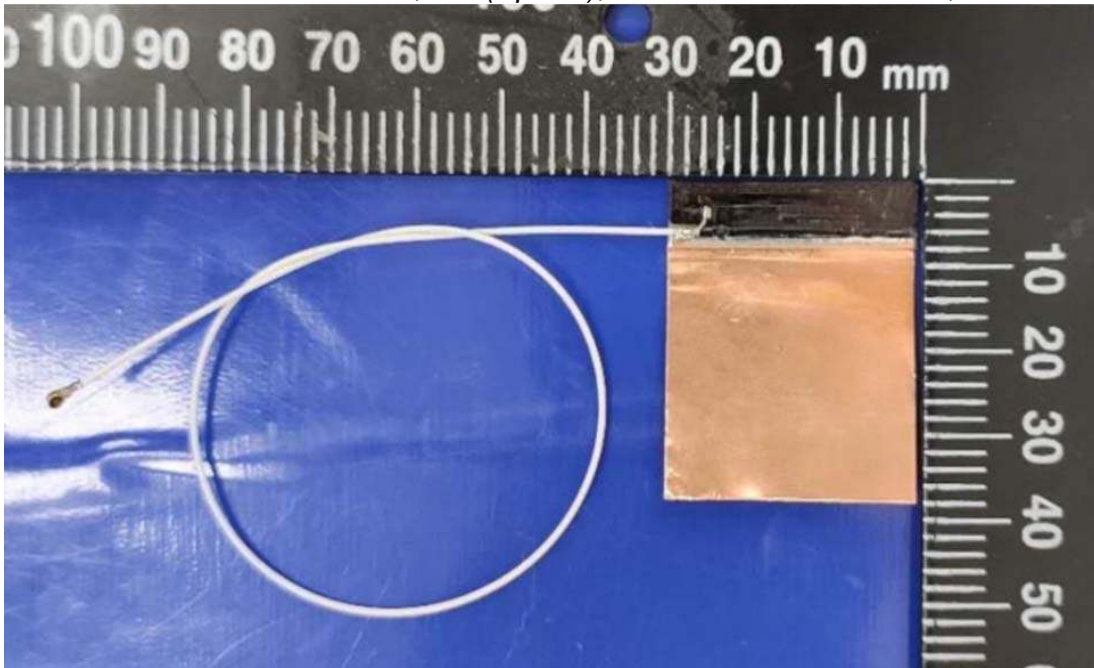
Figure 54 AUX, LG (Speed), WLAN Combo Antenna, Front View
