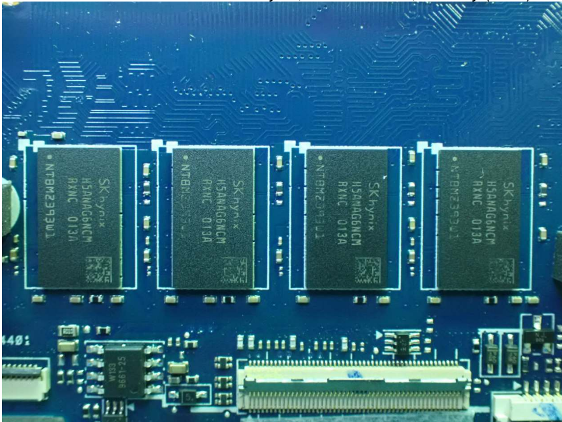
Figure 36 SK Hynix, 16GB View #1, Memory (RAM) View
