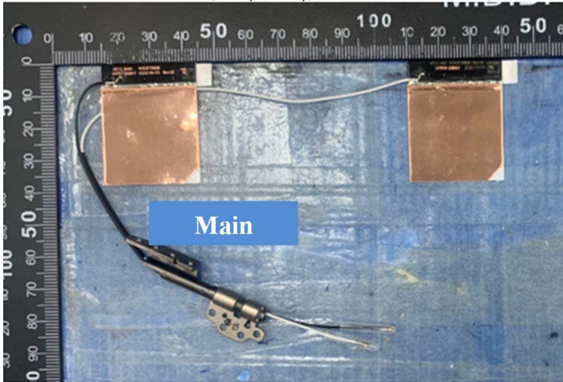
Figure 48 Main, LG (AWAN), WLAN Combo Antenna, Front View
