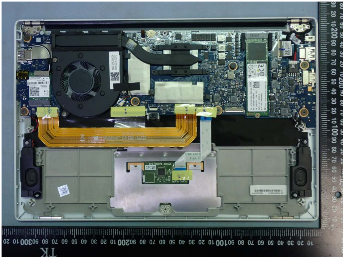
Figure 20 Internal View
