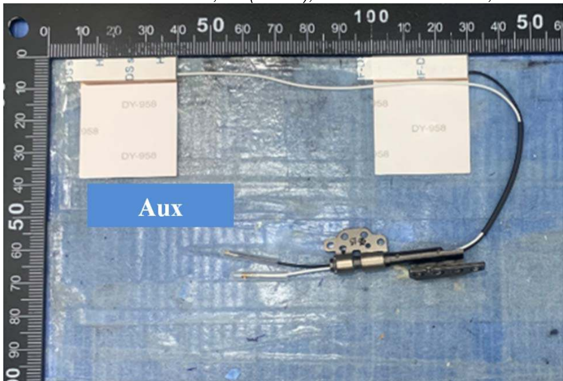
Figure 51 AUX, LG (AWAN), WLAN Combo Antenna, Back View
