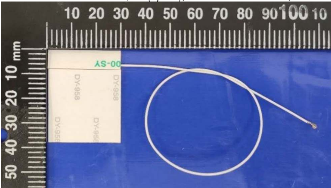
Figure 55 AUX, LG (Speed), WLAN Combo Antenna, Back View
