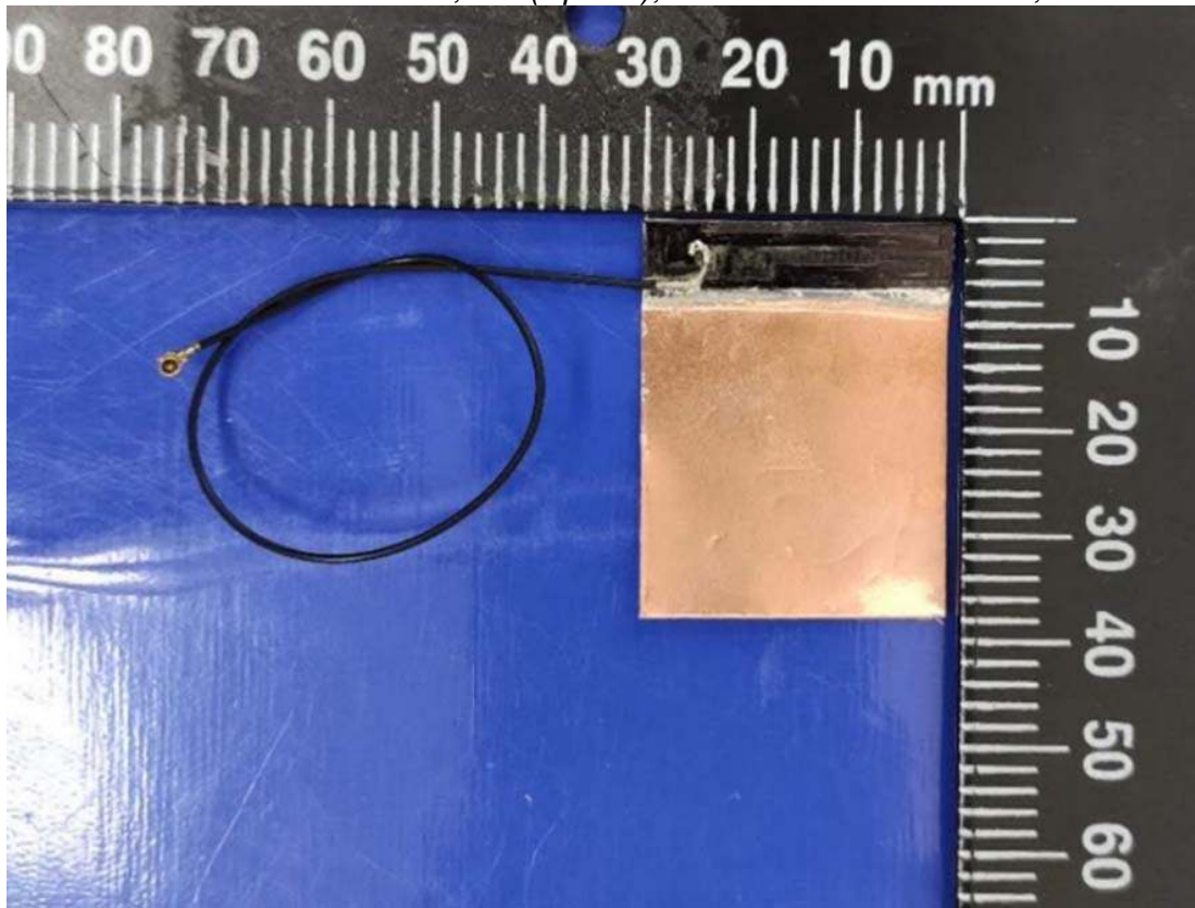
Figure 52 Main, LG (Speed), WLAN Combo Antenna, Front View
