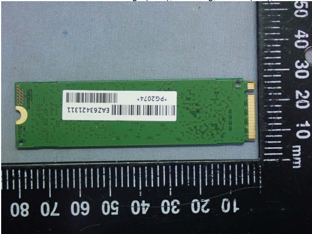
Figure 33 Storage (SSD), Samsung, 512GB (M.2), Back View
