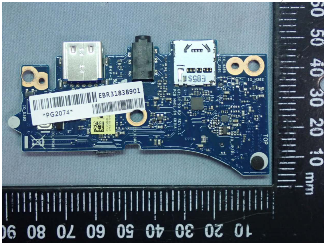
Figure 29 WLAN SUB Board, Back View
