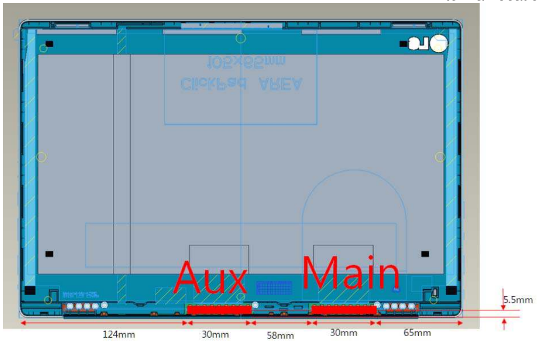
Figure 21 Antenna Location
