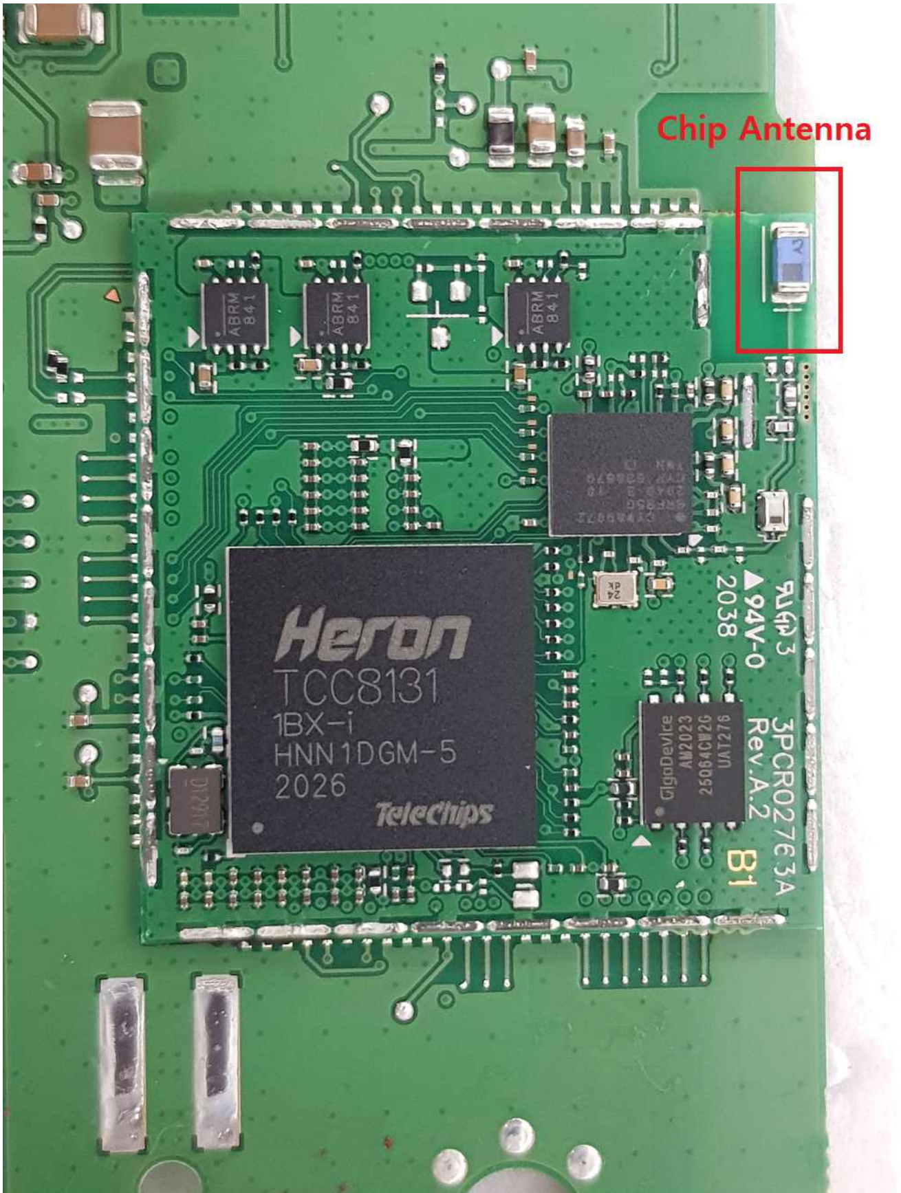
[BT Module_Right_Ant (Chip Antenna)]
