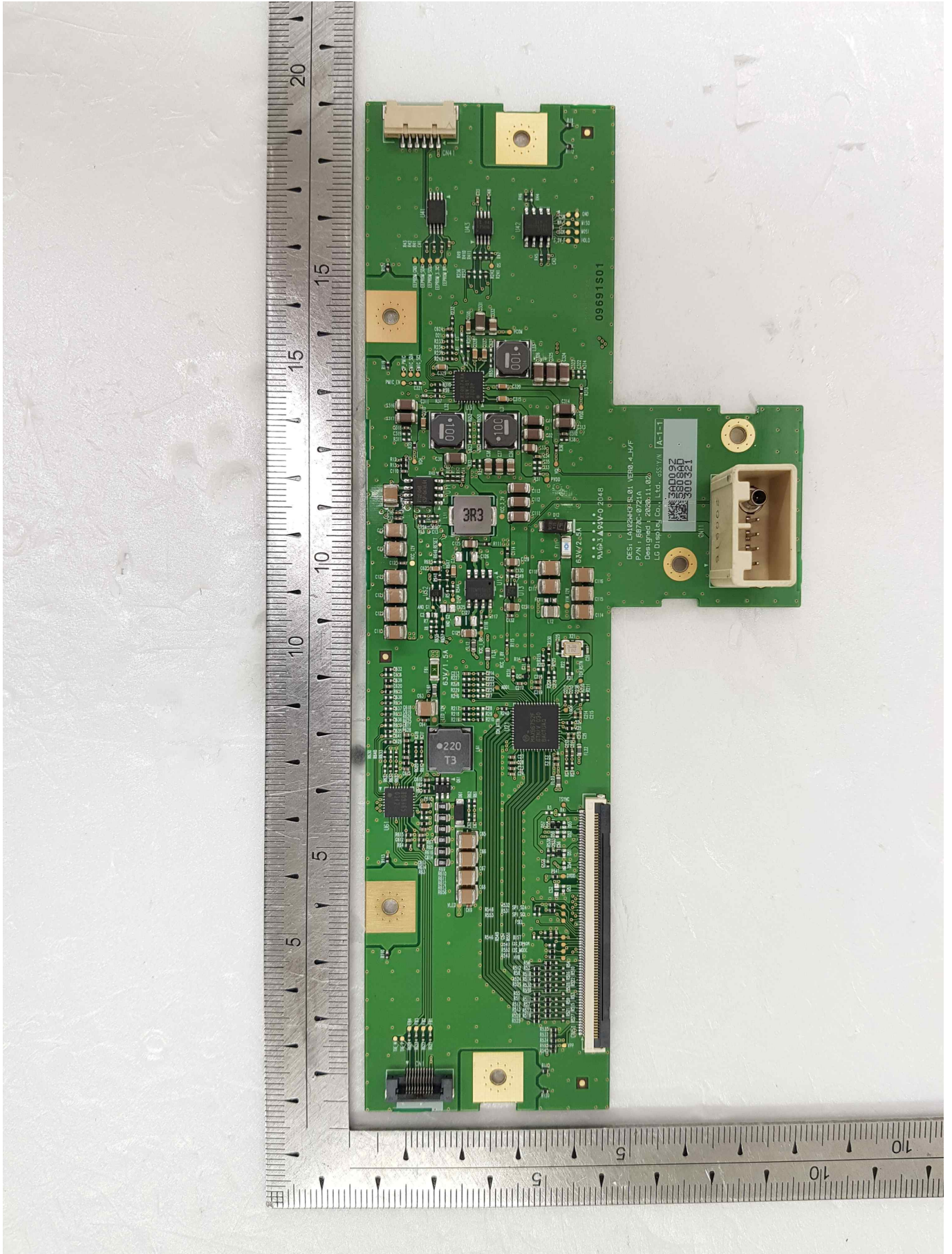
[Sub Board_Front]
