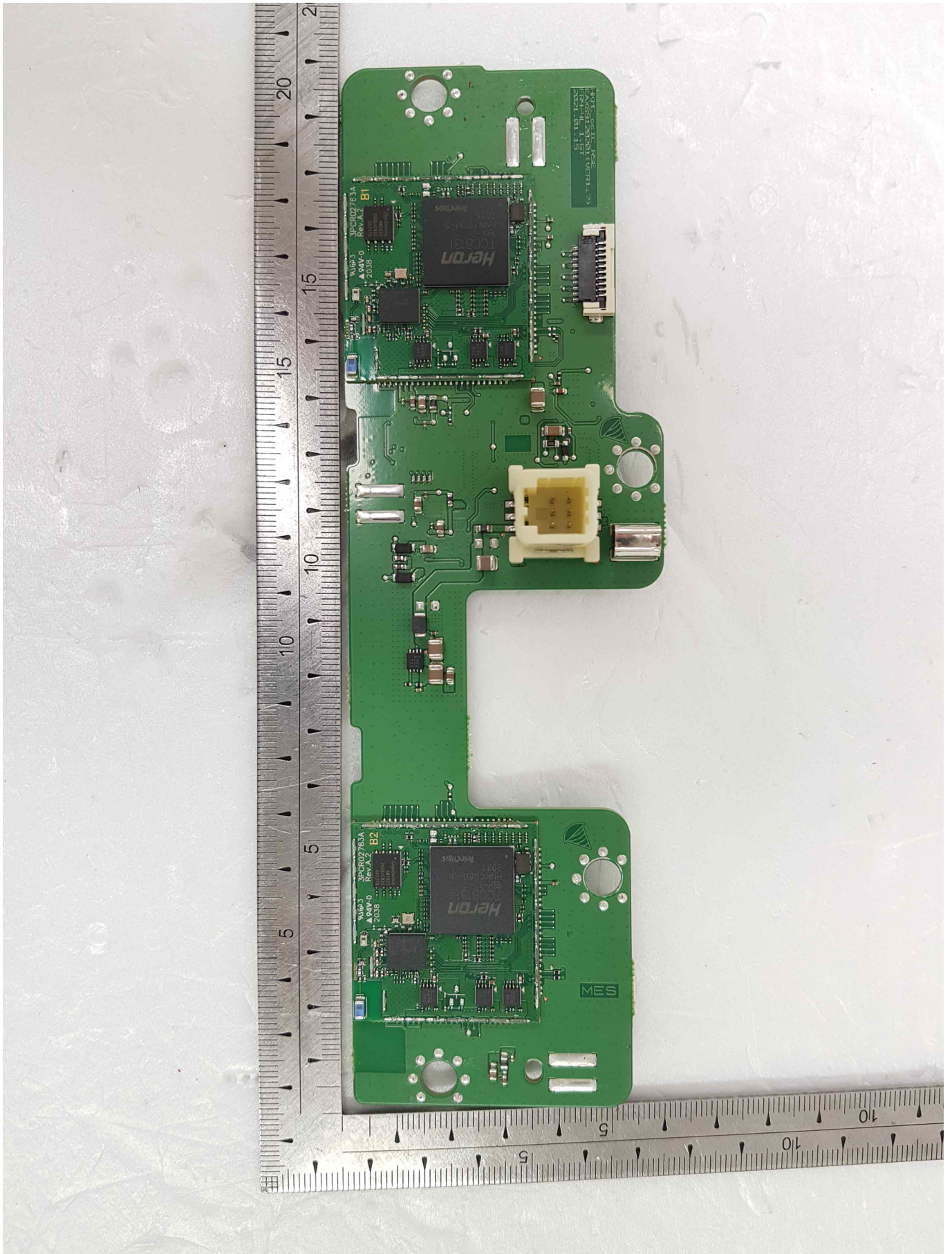
[Main Board(Shield Can Remove)_Front]
