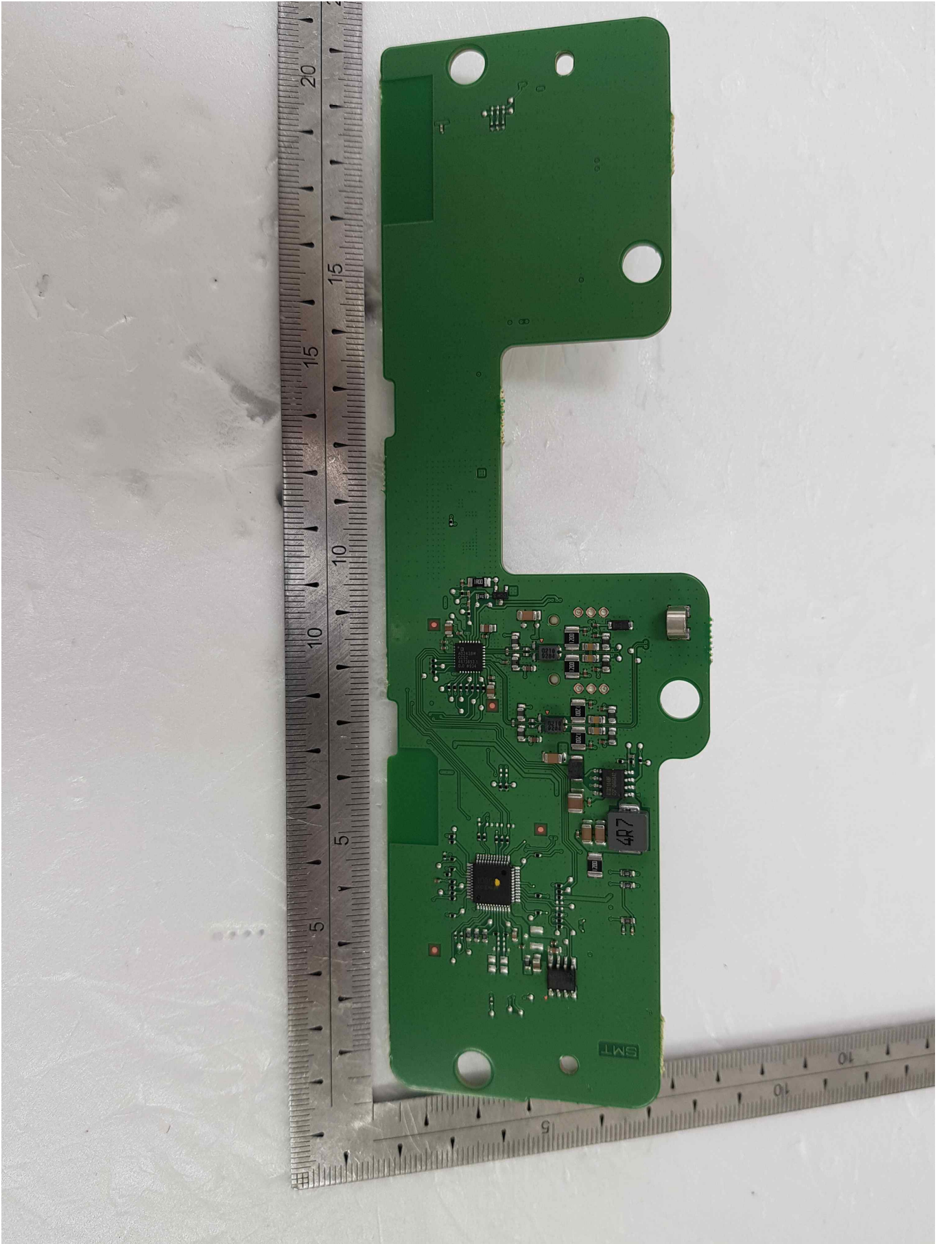
[Main Board_Rear]
