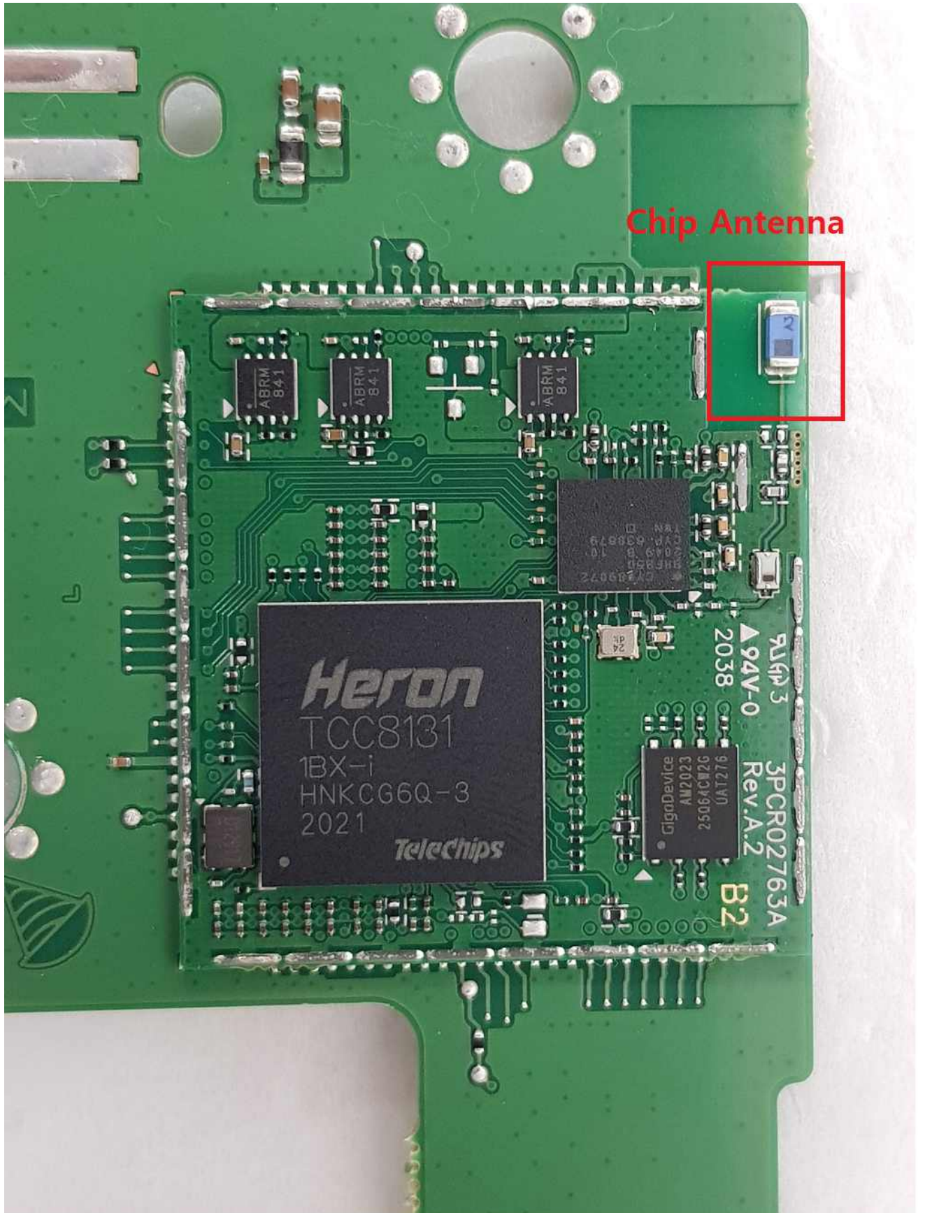
[BT Module_B2_Left (Chip Antenna)]
