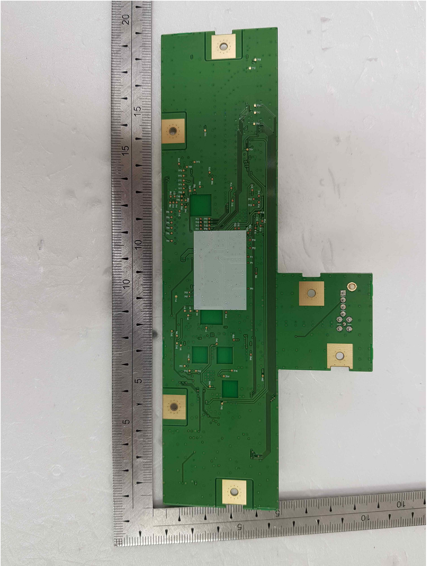
[Sub Board_Rear]
