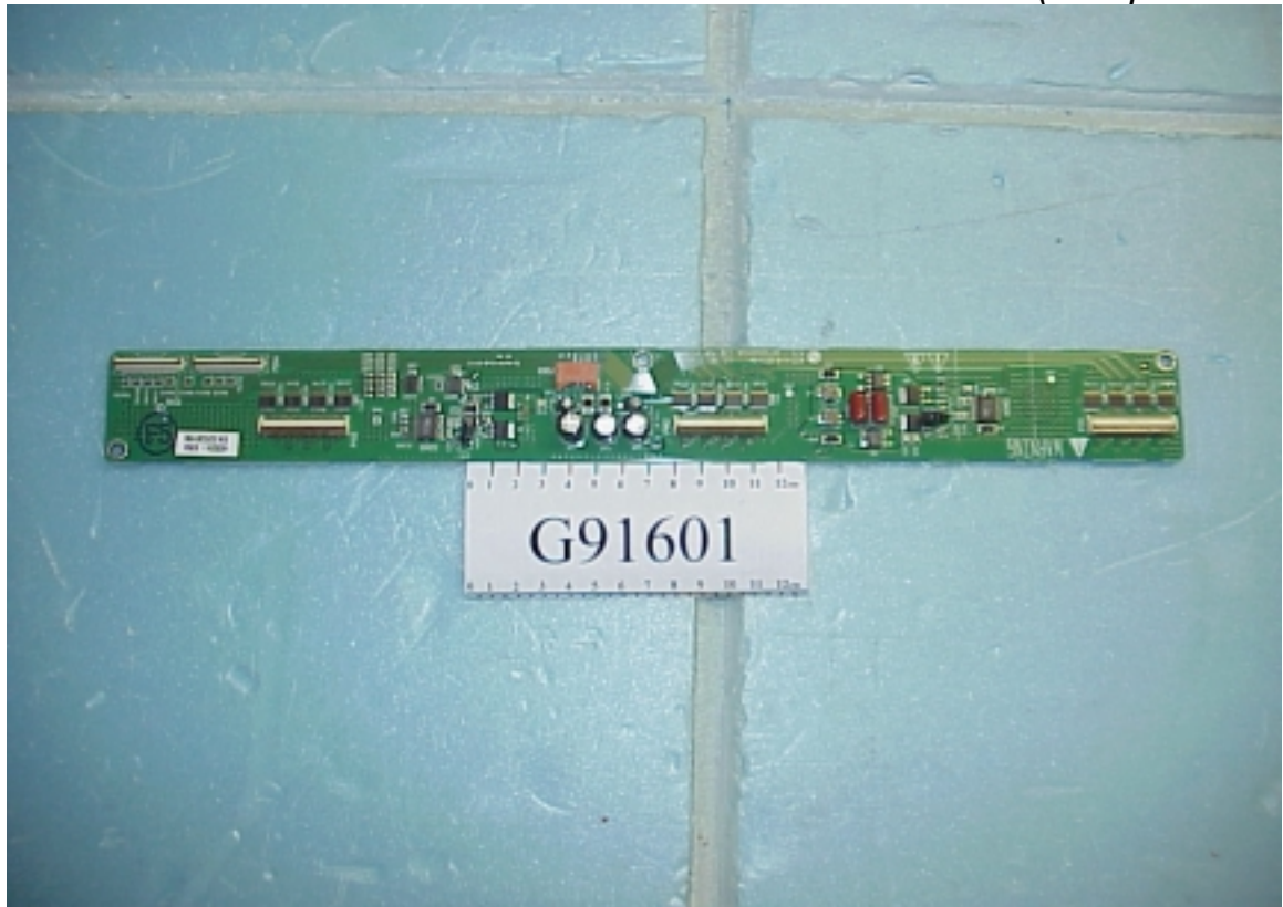
Figure 29 X-Drive Board #1 (Component Side)
