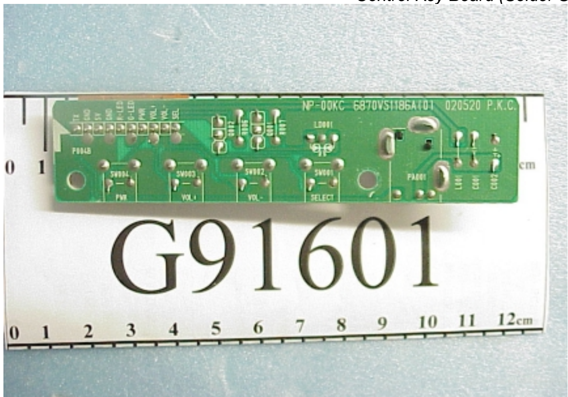
Figure 34 Control Key Board (Solder Side)
