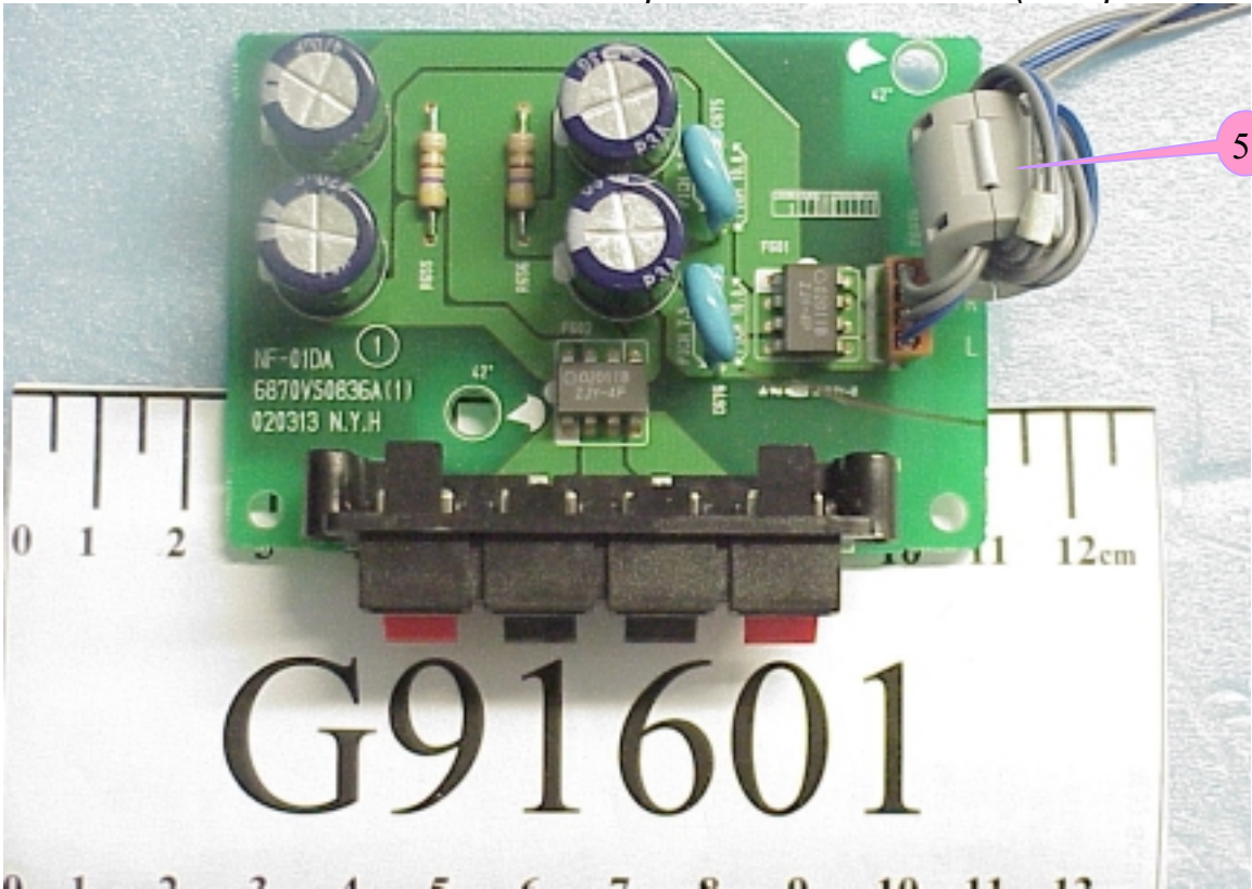
Figure 38 Speaker Control Board (Component Side)
