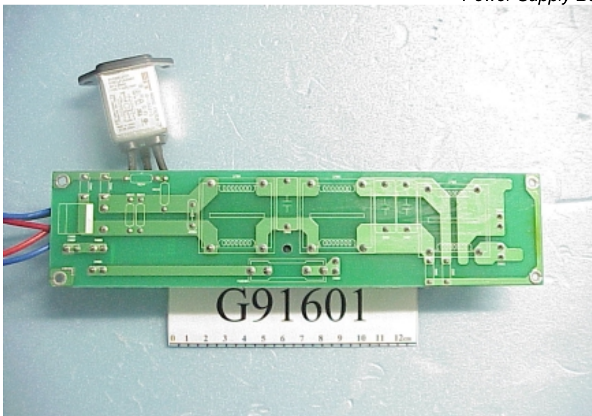
Figure 42 Power Supply Board
