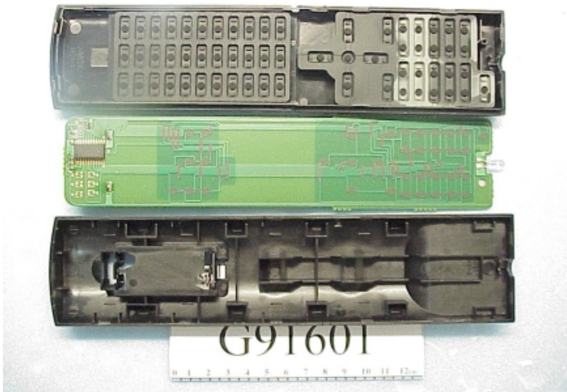
Figure 52 Remote Control (Internal View)
