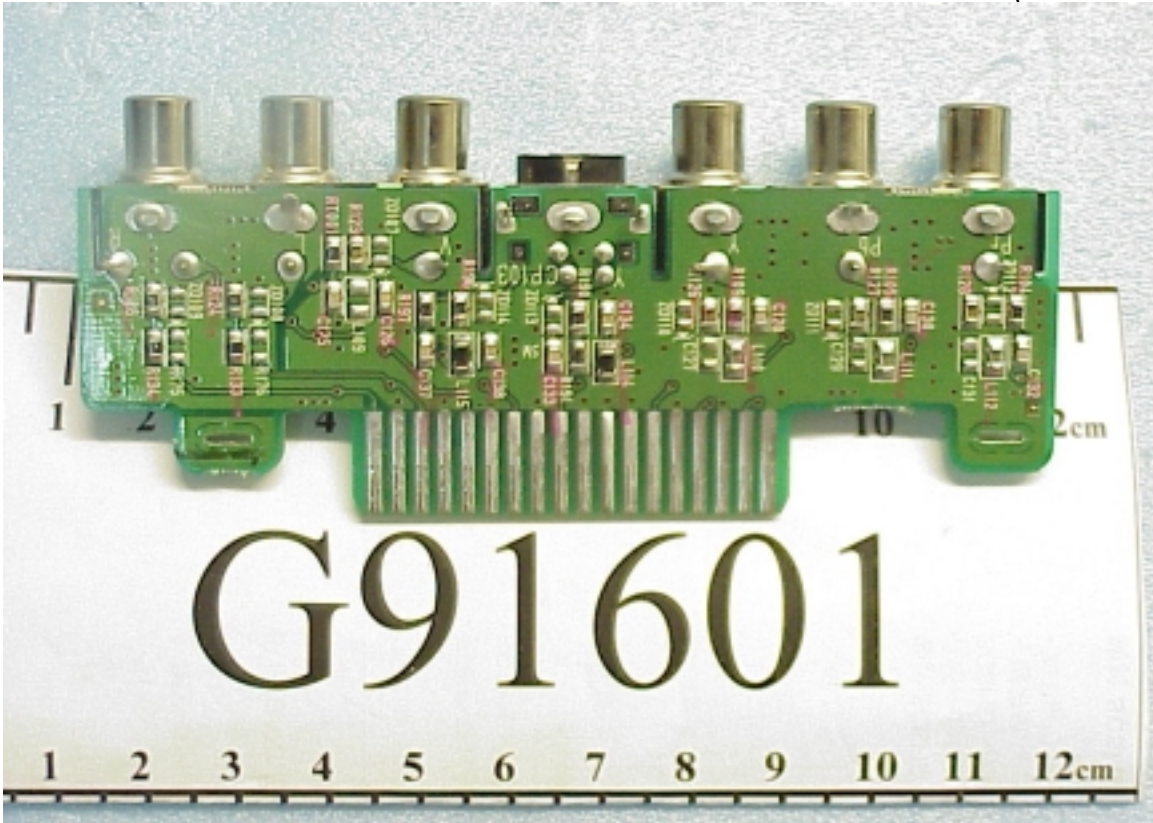
Figure 37 Video Board (Solder Side)
