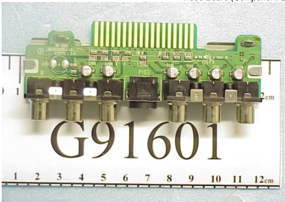
Figure 36 Video Board (Component Side)
