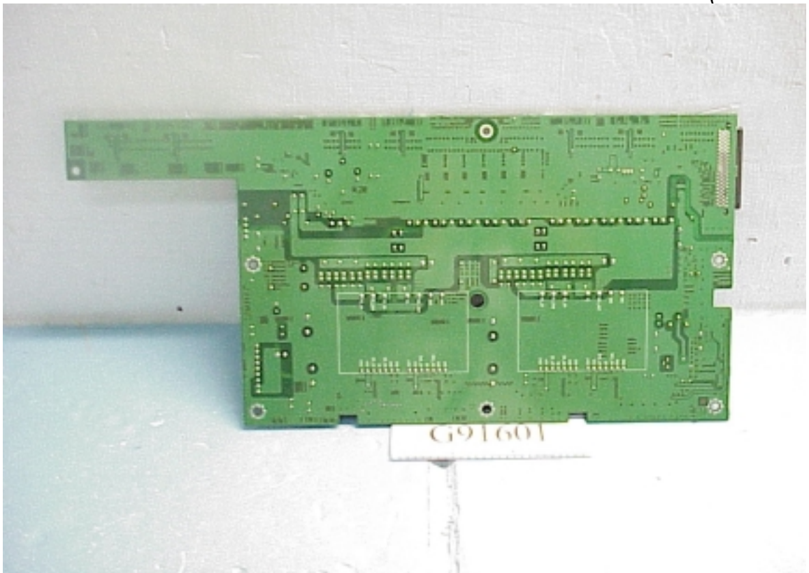
Figure 14 Y Board (Solder Side)
