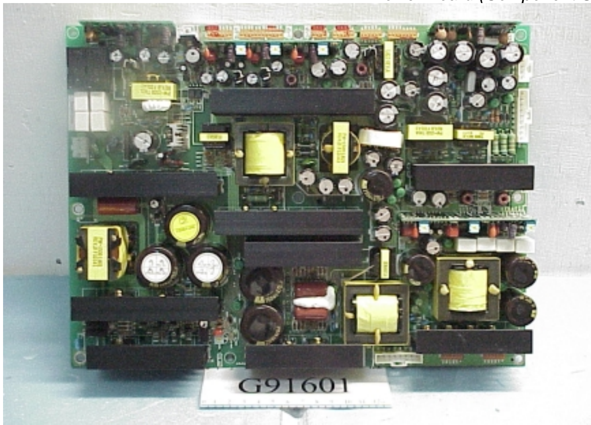
Figure 17 Power Board (Component Side)
