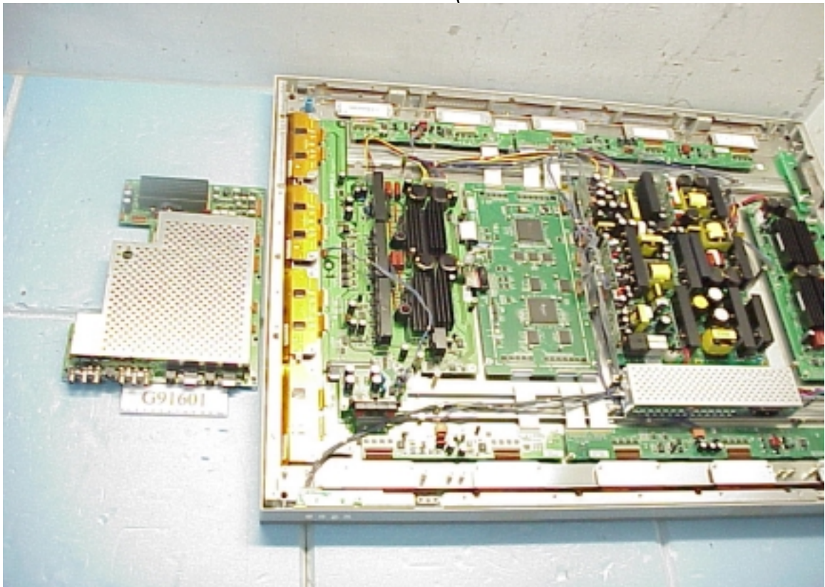
Figure 7 Internal View (Remove Main Board w/ Metal Cover)
