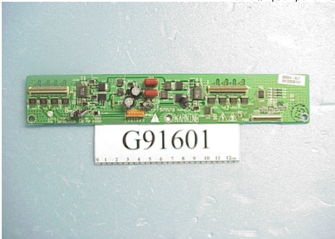
Figure 23 X Board #1 (Component Side)
