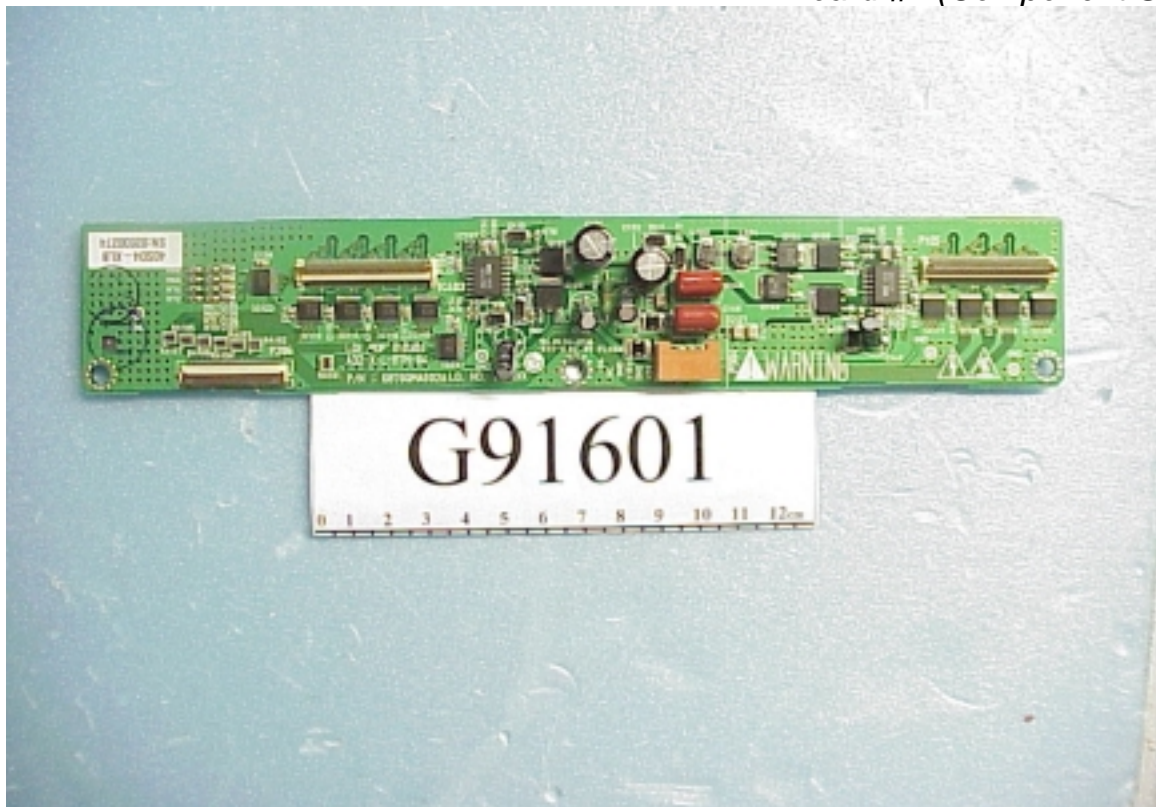
Figure 27 X Board #2 (Component Side)
