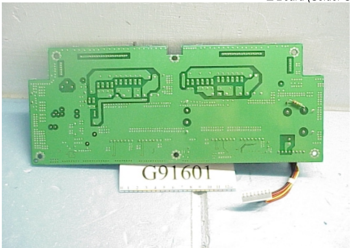
Figure 20 Z Board (Solder Side)
