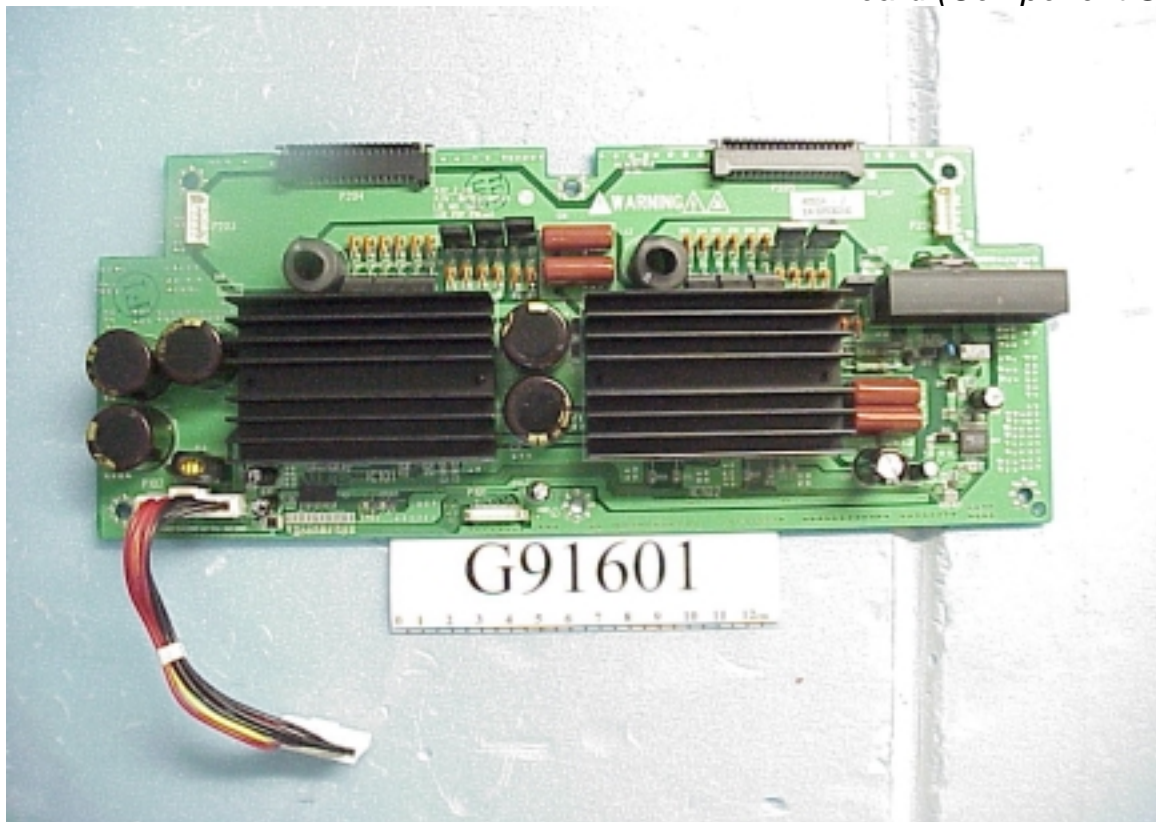
Figure 19 Z Board (Component Side)
