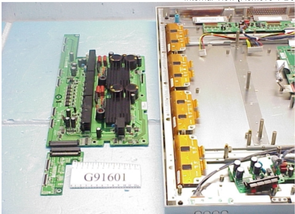
Figure 12 Internal View (Remove Y Board)
