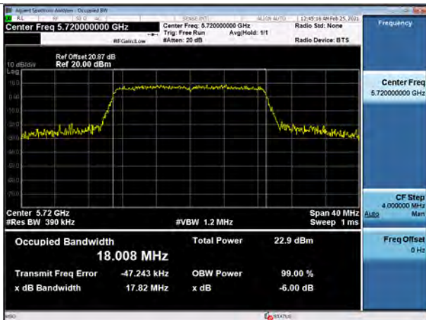
802.11ac_VHT20 UNII 2C (CH 144)
