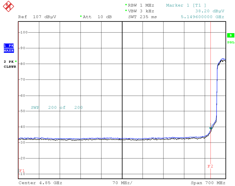
Average Reading (802.11n(HT40), Ch.38, X-H)
