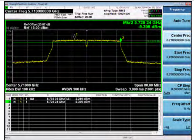
802.11ac_VHT40 CH.142
