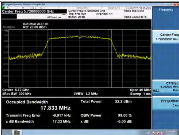
802.11n_HT20 UNII 2C (CH 144)
