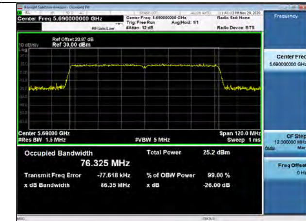
802.11ac_VHT80 UNII 2C (CH 138)
