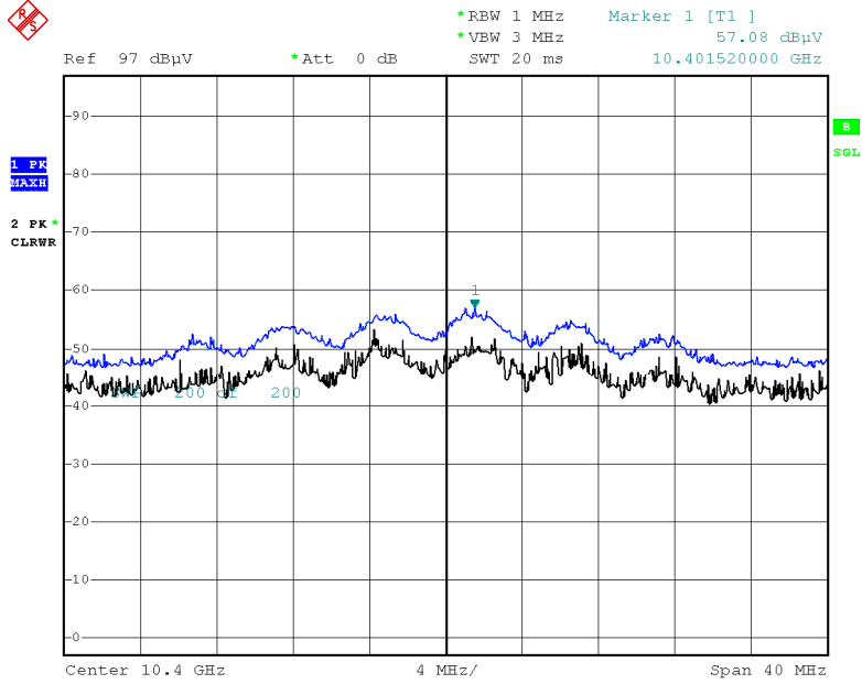
Peak Reading (802.11a, Ch.40 2nd Harmonic, H)
