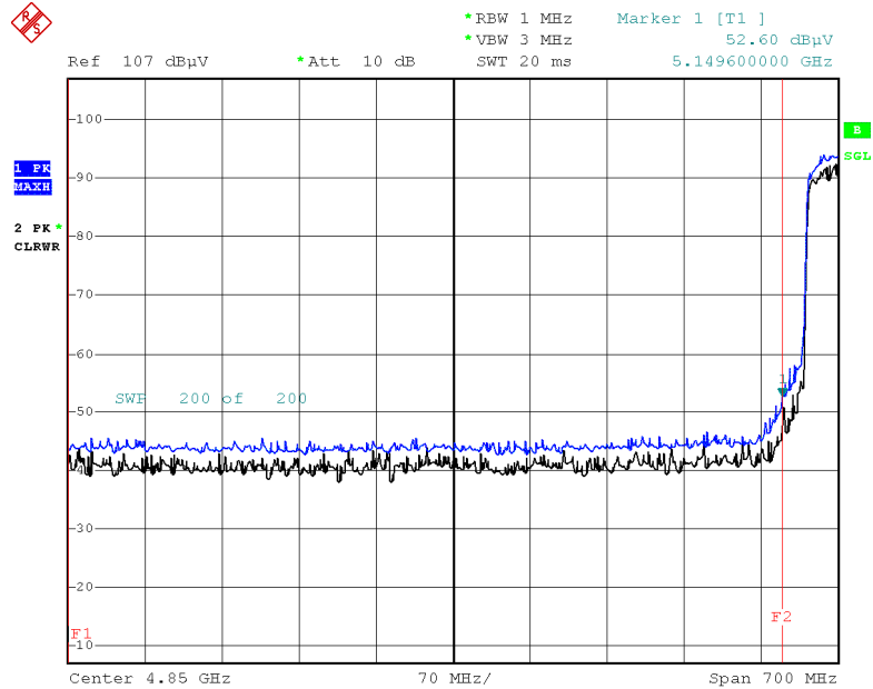
Peak Reading (802.11n(HT40), Ch.38, X-H)
