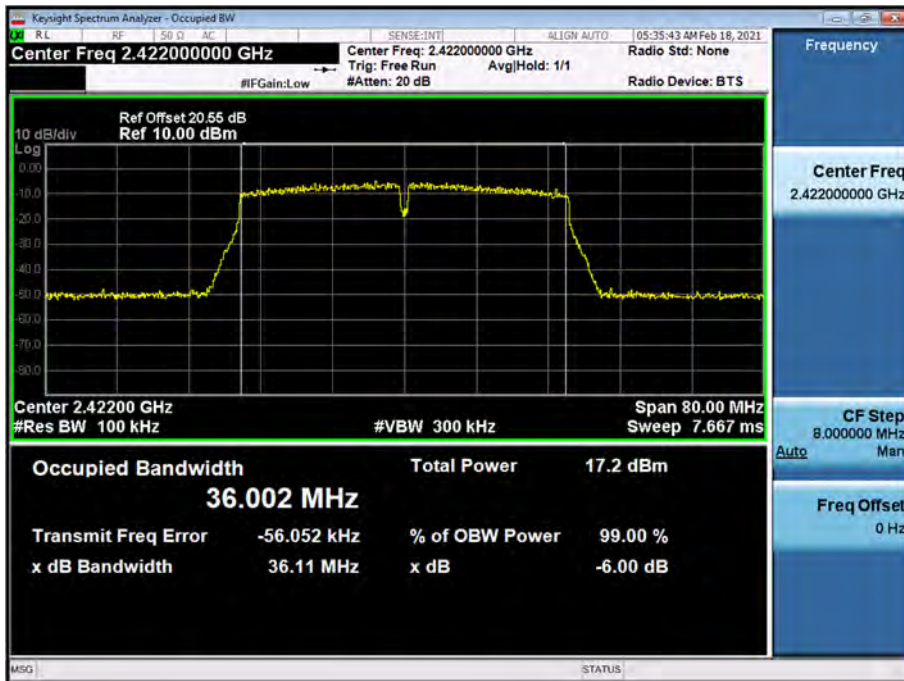
6dB Bandwidth plot (802.11n_HT40-CH 1)
