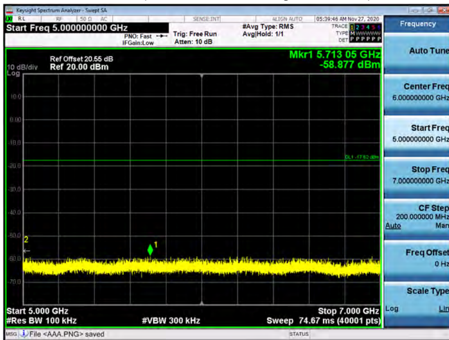
Conducted Spurious Emission (802.11g_Ch.11_54 Mbps)
