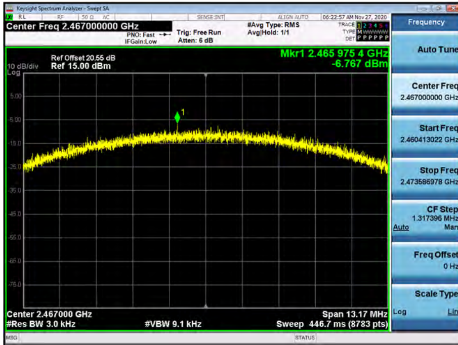
Power Spectral Density (802.11b-CH 12)
