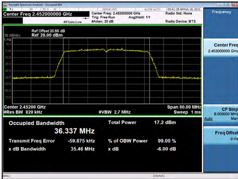
99% Bandwidth plot (802.11n_HT40-CH 9)
