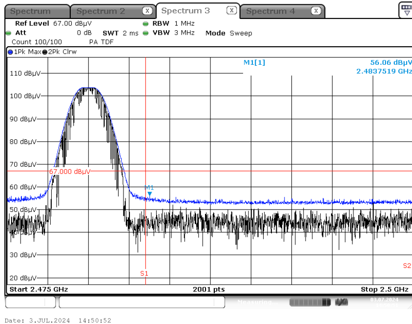
Radiated Restricted Band Edges plot – Peak Result (Ch.39, Y-V)
