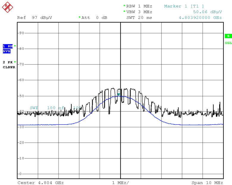
Radiated Spurious Emissions plot – Average Result (Ch.0 2nd Harmonic, Y-H)
