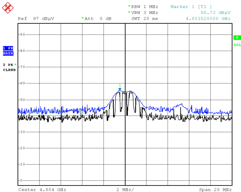
Radiated Spurious Emissions plot – Peak Result (Ch.0 2nd Harmonic, Y-H)
