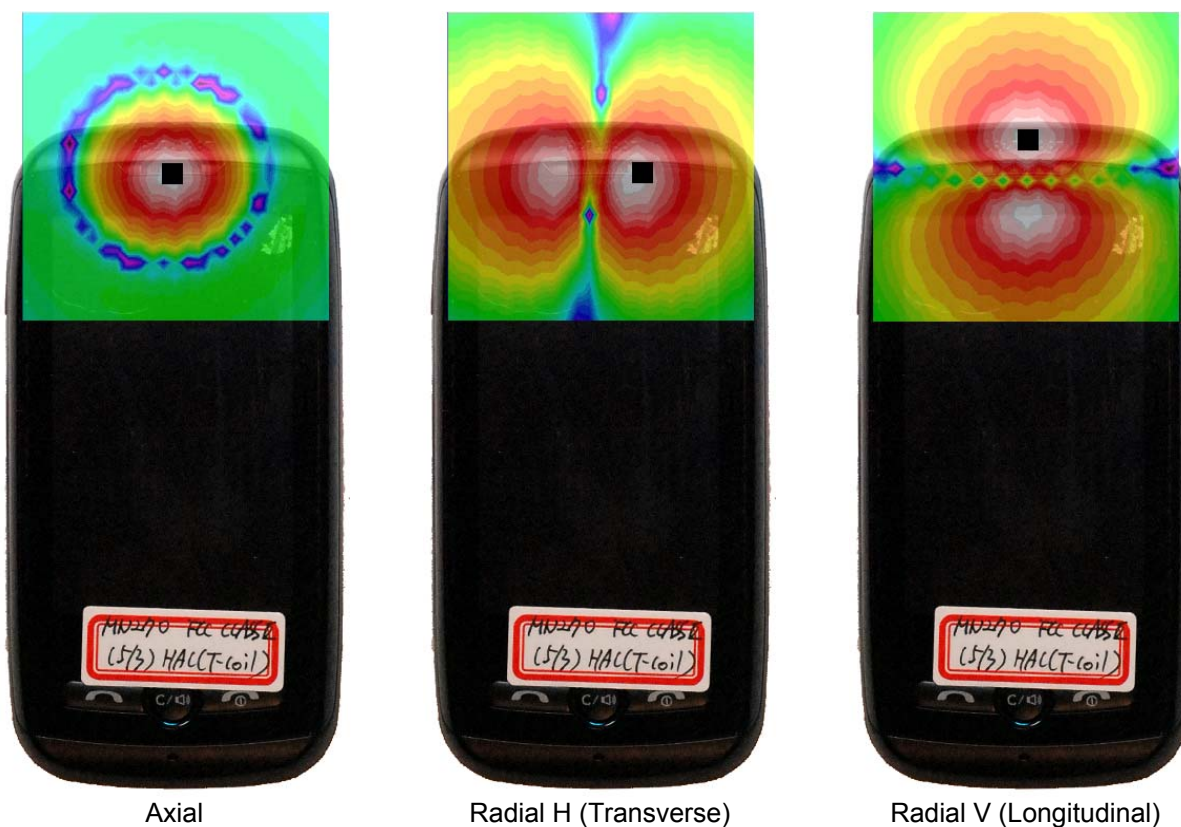
Figure 13-3 T-Coil Scan Overlay Magnetic Field Distributions
