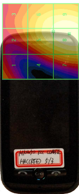
Figure 17-4 E-Field WD Scan overlay
