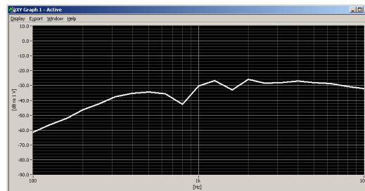
Figure 6-2 Worst-case ABM2 Plot for WD
