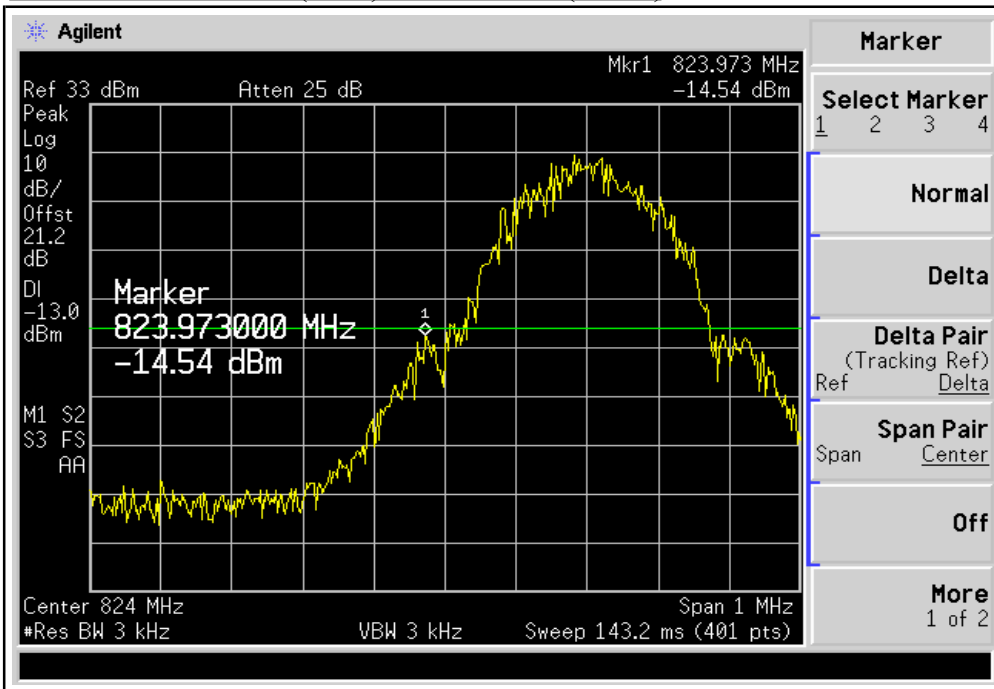
PLOTS OF EMISSION (GSM): BAND EDGE(Ch128)
