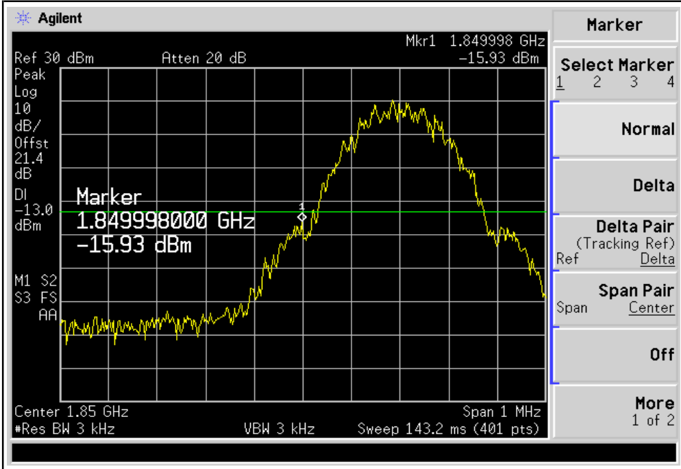
PLOTS OF EMISSION (CDMA): BAND EDGE(Ch512)
