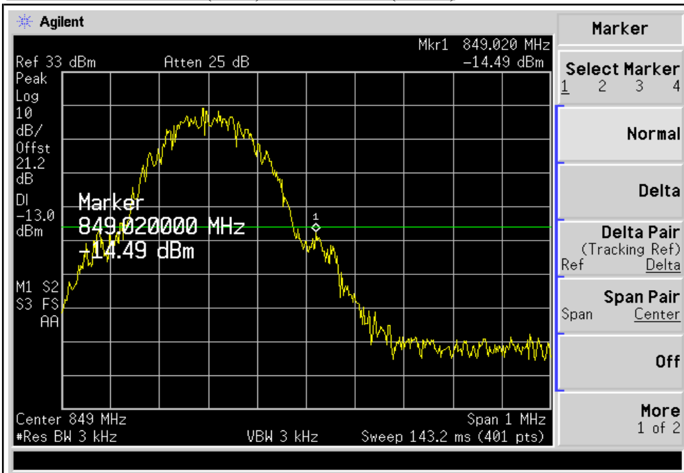
PLOTS OF EMISSION (GSM): BAND EDGE(Ch251)
