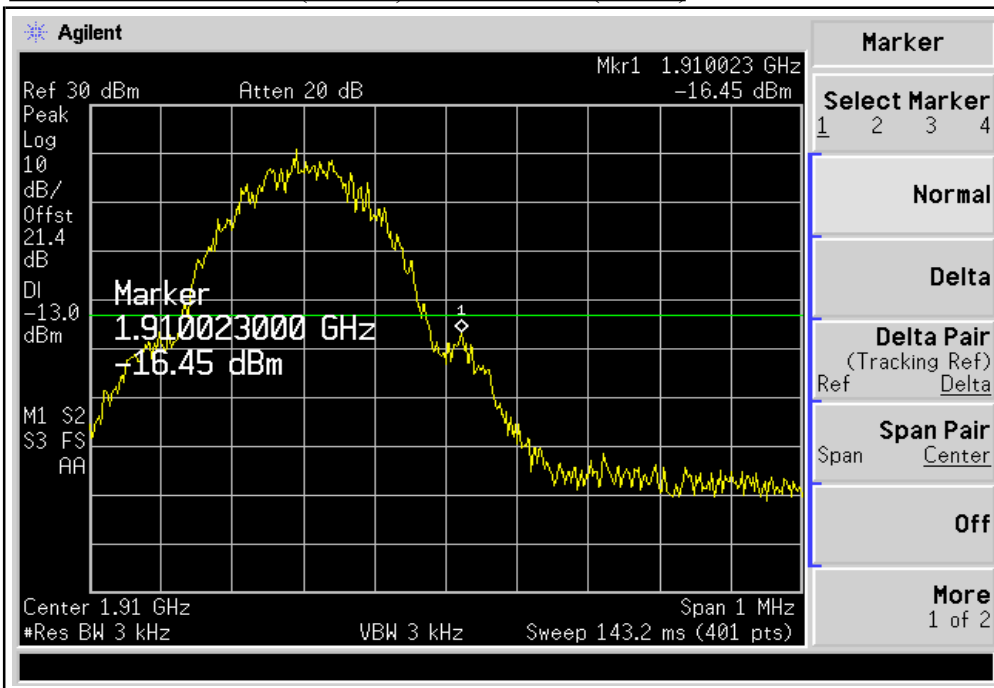
PLOTS OF EMISSION (CDMA): BAND EDGE(Ch810)
