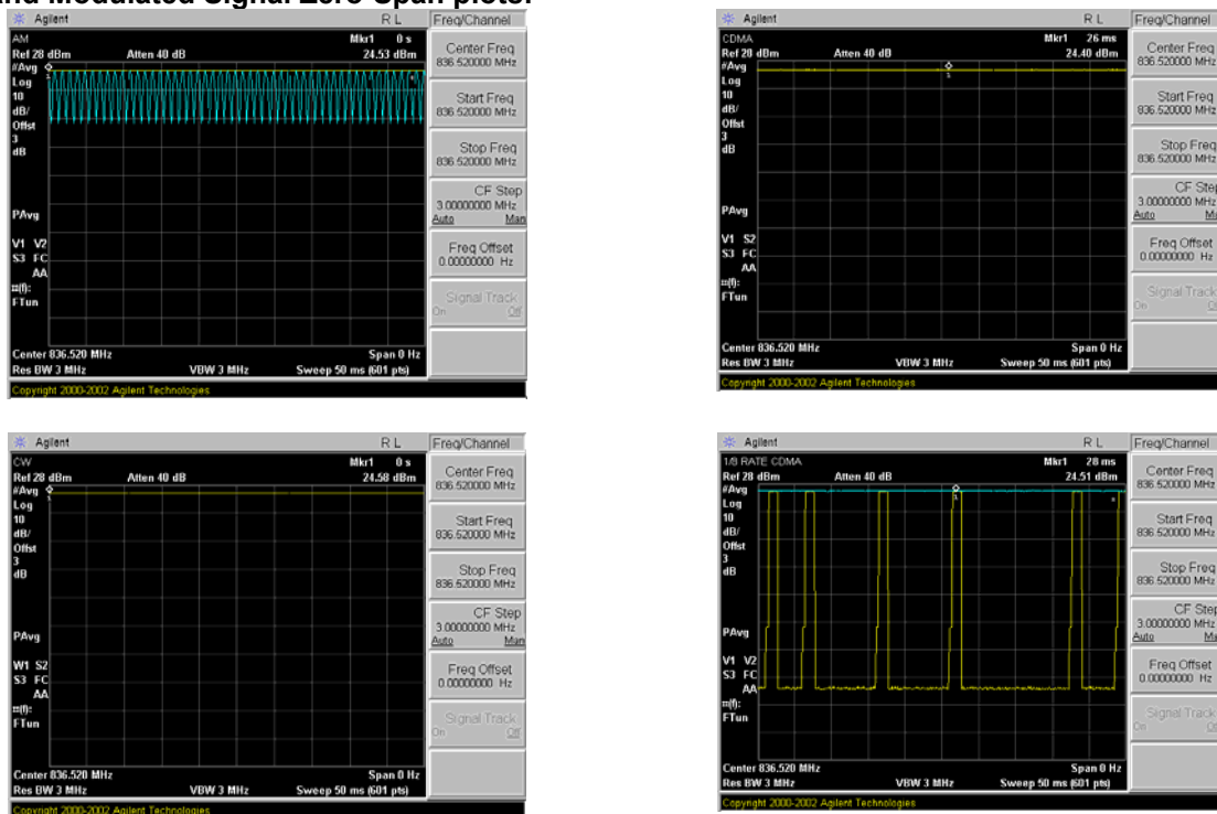
Figure 22 Zero-Span Plots
