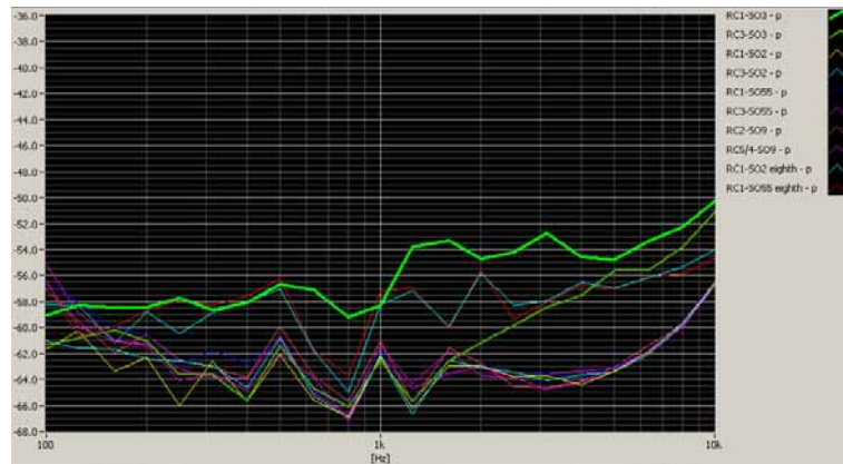
Figure 7-1 CDMA2000 Audio Band Magnetic Noise
