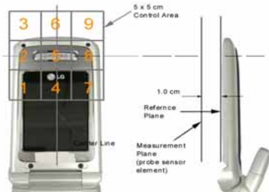
Figure 13 E/H-Field Emissions Test Setup Diagram
