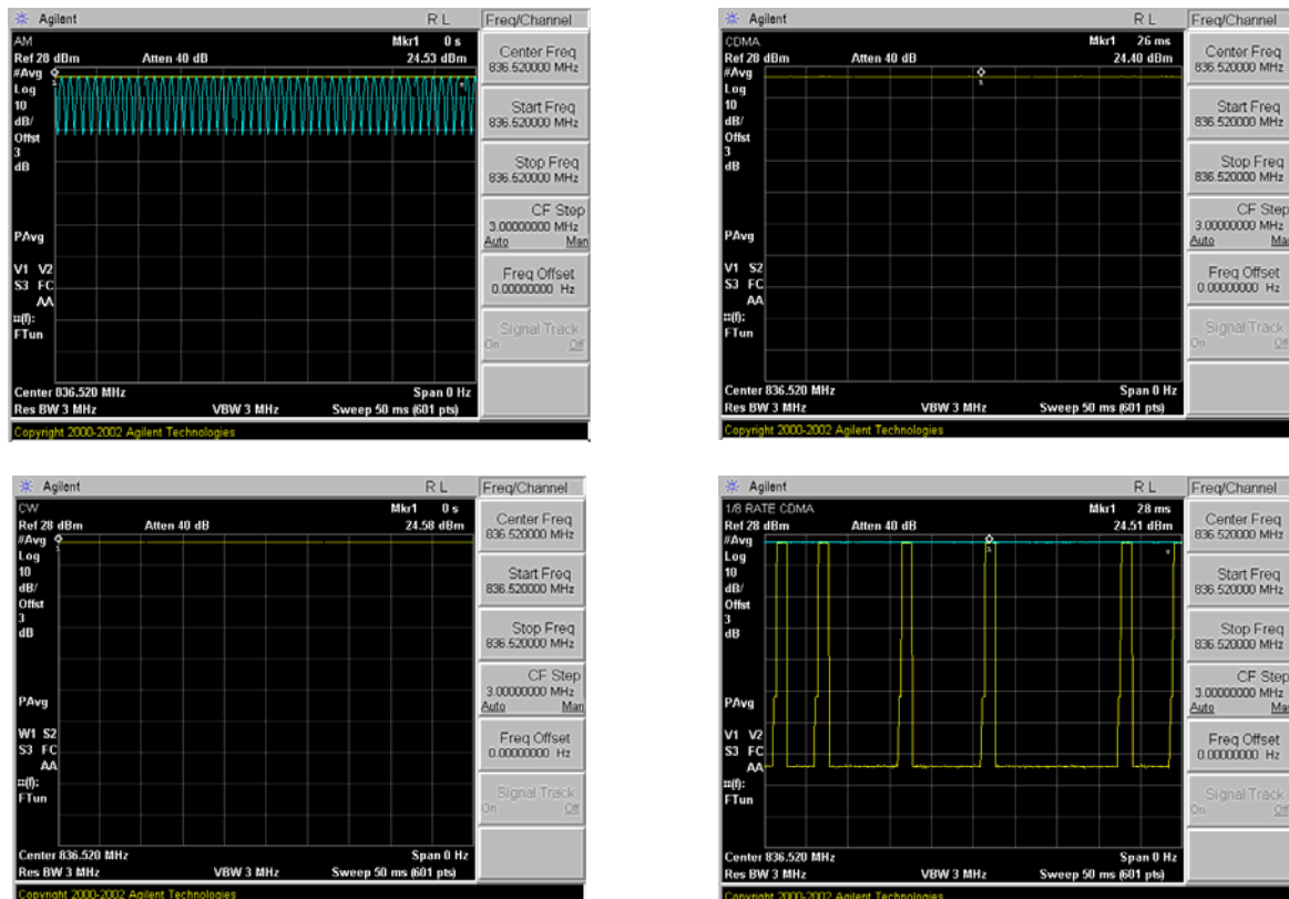
Figure 26 Zero-Span Plots
