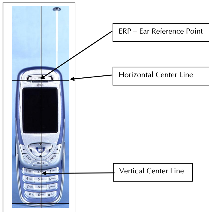
Figure 13.1 Handset Reference Points
