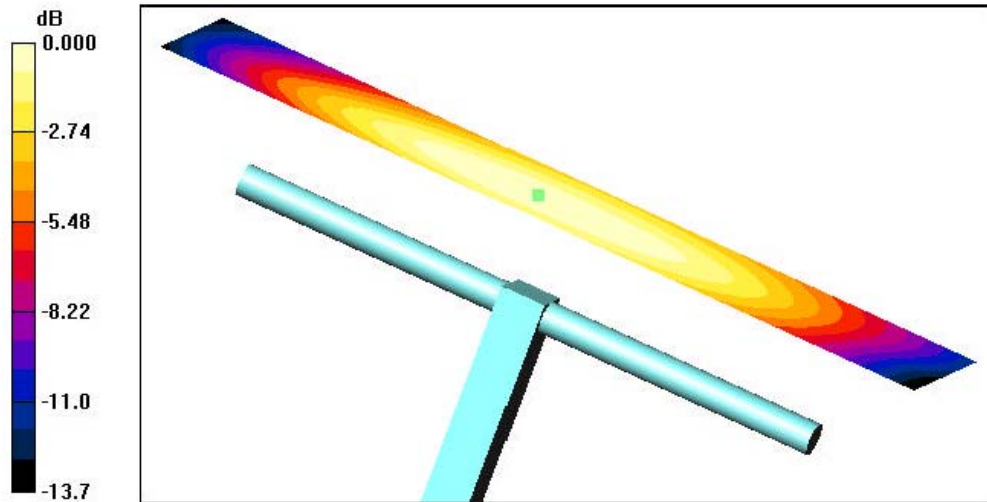
0 dB = 0.410A/m
