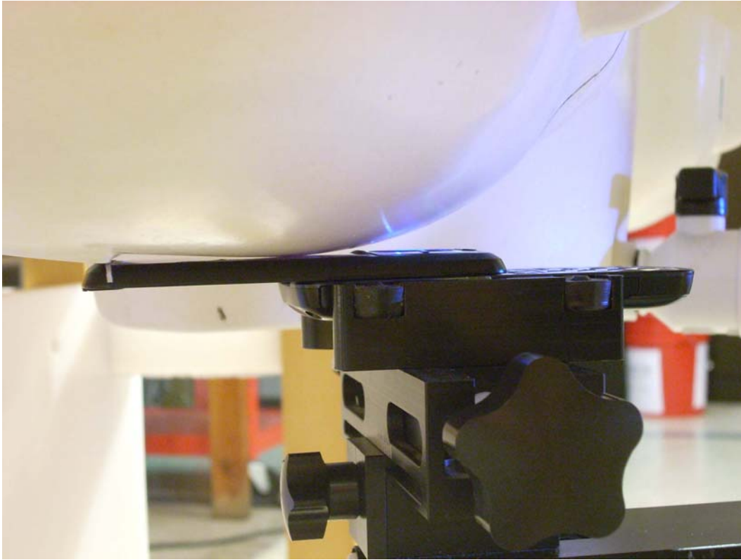
Figure 5: Right Head SAR, Cheek Touch, Slide Out
