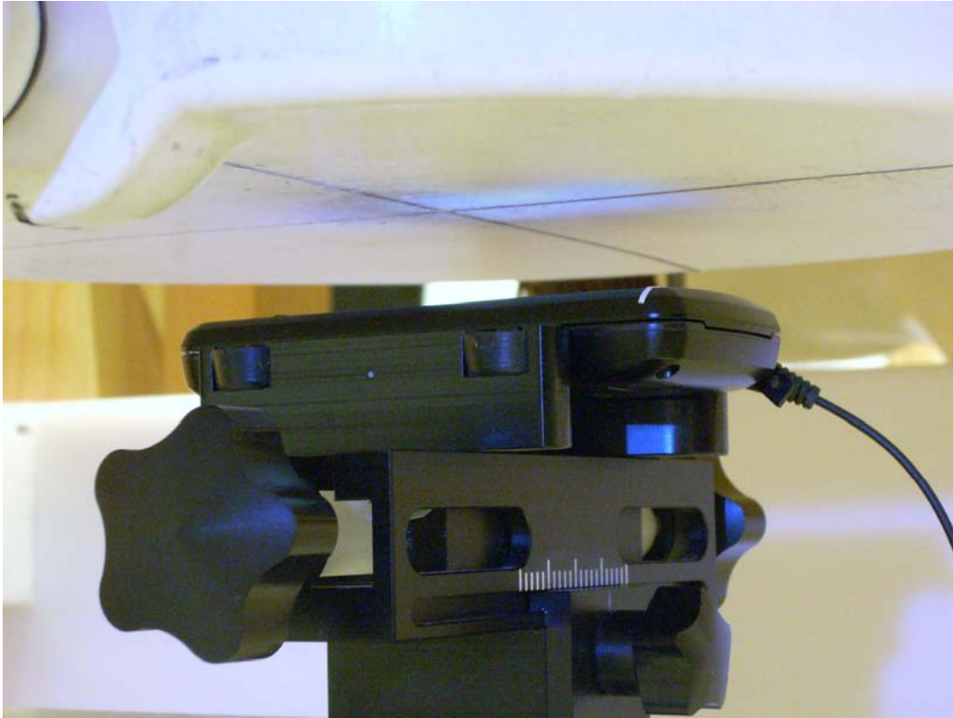
Figure 13: Body SAR, Front Side with 20mm Space
