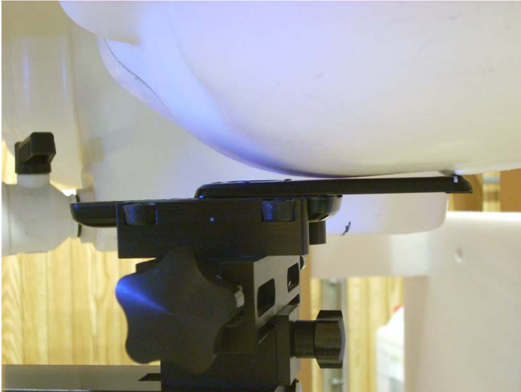
Figure 9: Left Head SAR, Cheek Touch, Slide Out
