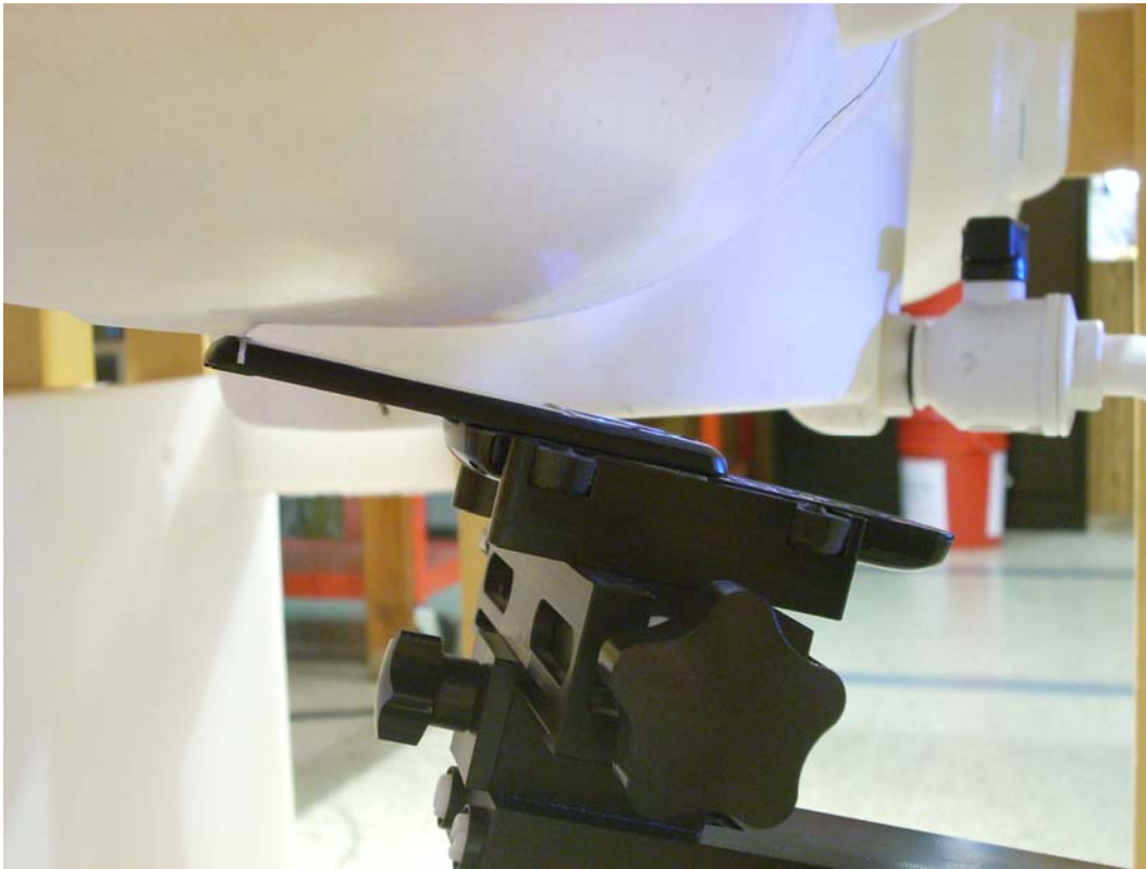
Figure 6.: Right Head SAR, 15° Tilt, Slide Out
