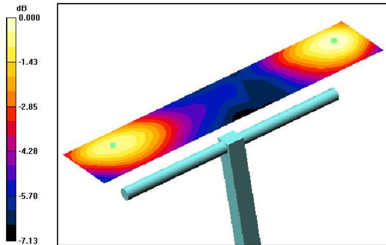
0 dB = 136.8V/m
