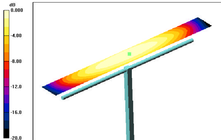
0 dB = 0.433A/m
