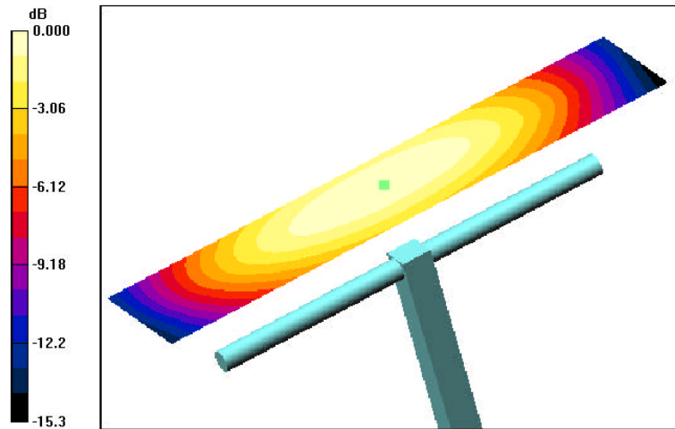
0 dB = 0.429A/m
