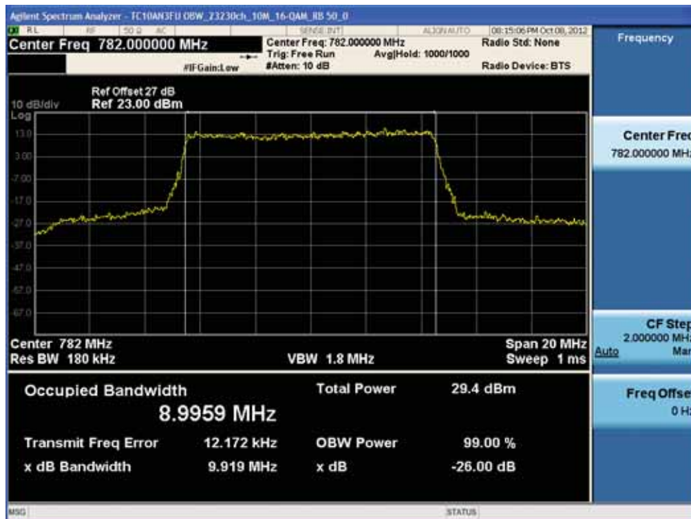
BAND 13. Occupied Bandwidth Plot (23230ch_10MHz_16-QAM_RB 50)
