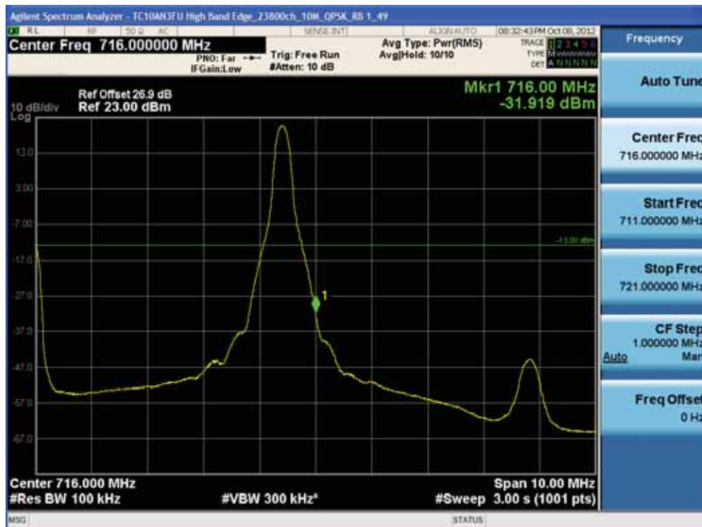
BAND 17. High Band Edge Plot (23800ch_10MHz_QPSK_RB 1_49)
