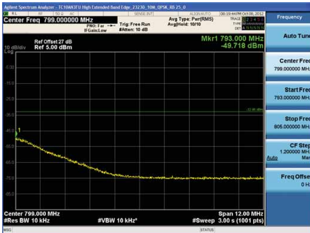
BAND 13. High Extended Band Edge Plot (23230ch_10MHz_QPSK_RB 25_0)
