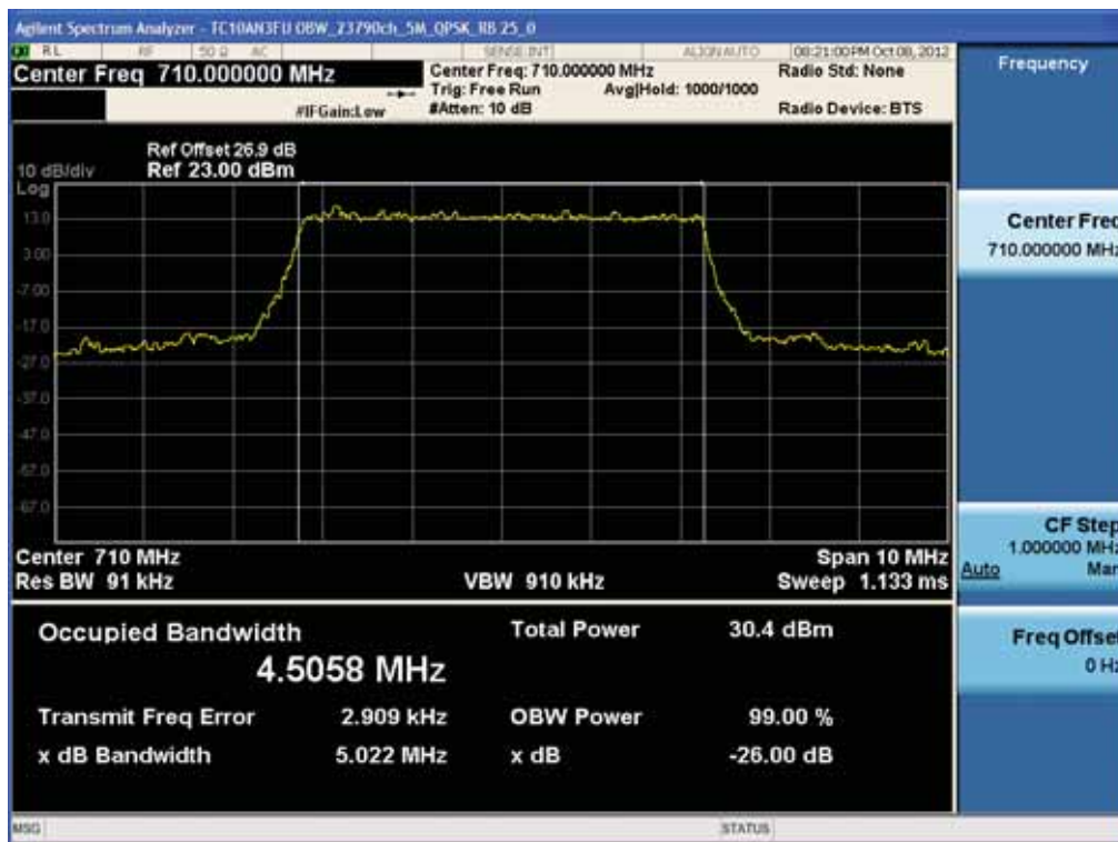
BAND 17. Occupied Bandwidth Plot (23790ch_5MHz_QPSK_RB 25)
