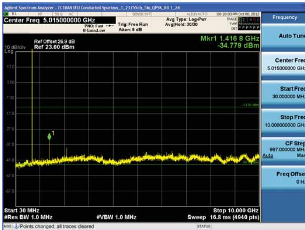
BAND 17. Conducted Spurious Plot_1 (23755ch_5MHz_QPSK_RB 1_24)
