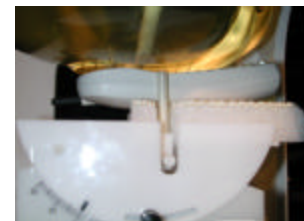
Fig. 14 Head SAR Test Setup
