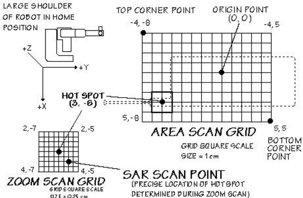
Figure 7. SAR Measurement Points in Area Scan and Zoom Scan Grids Showing the Typical Hot Spot with respect to the Phone
