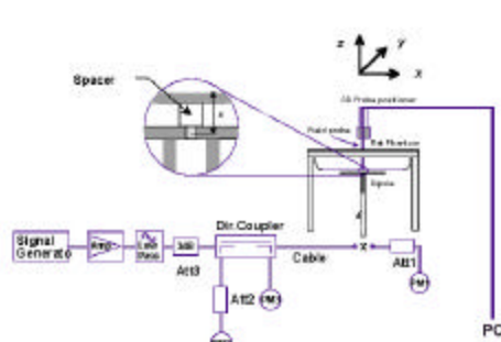
Figure 13.1 Dipole Validation Test Setup
