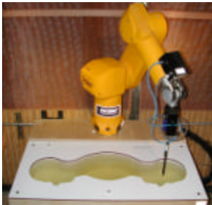
Figure 6.2 Simulated Tissue
