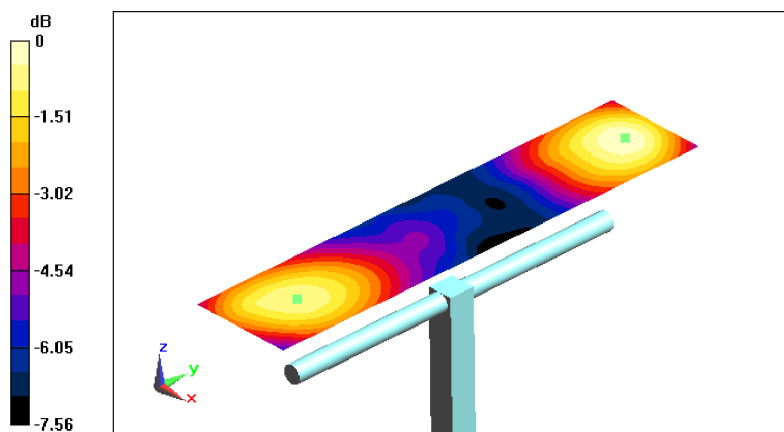
0 dB = 139.5V/m
