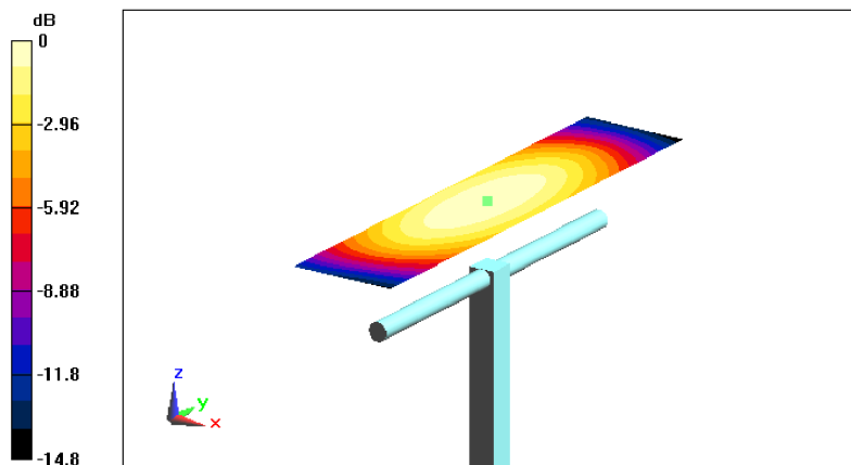
0 dB = 0.455A/m
