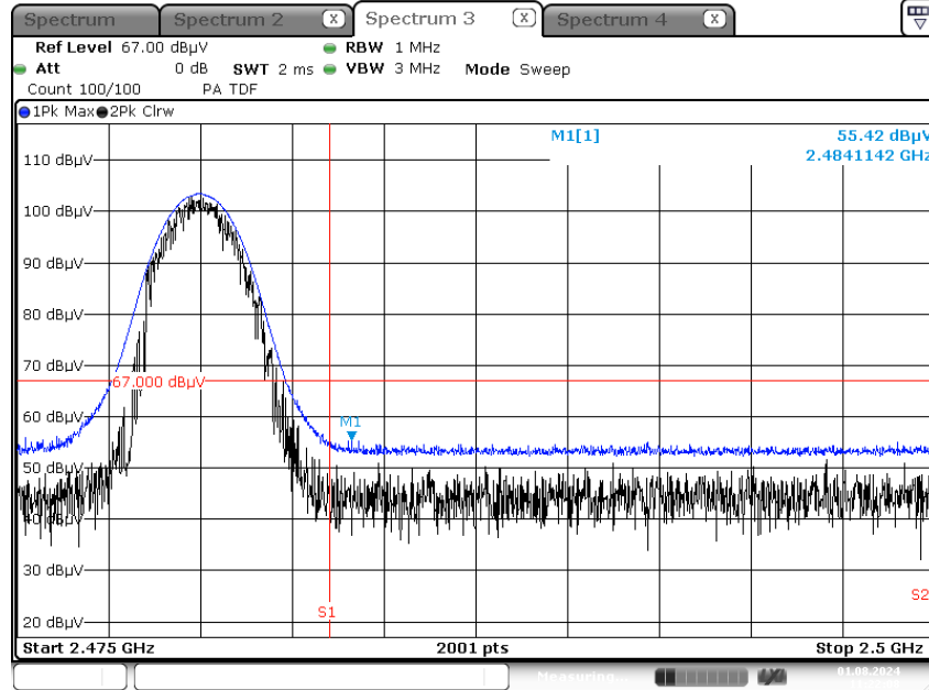
Radiated Restricted Band Edges plot – Average & Peak Result (8DPSK, Ch. 78, Y-V)
