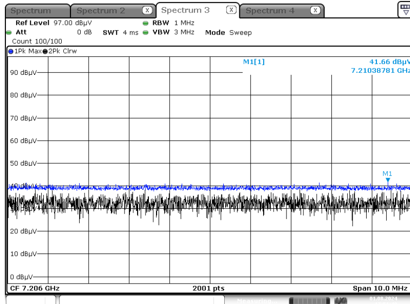
Radiated Spurious Emissions plot – Peak & Average Result (3rd Harmonic, Z-V)
