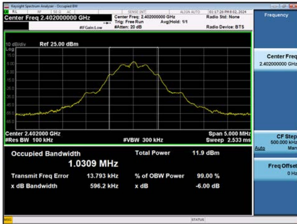
6 dB Bandwidth plot (Low-CH 0)
