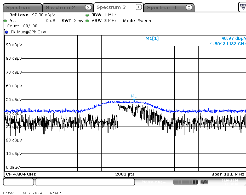
Radiated Spurious Emissions plot – Peak Result (Ch.0 2nd Harmonic)
