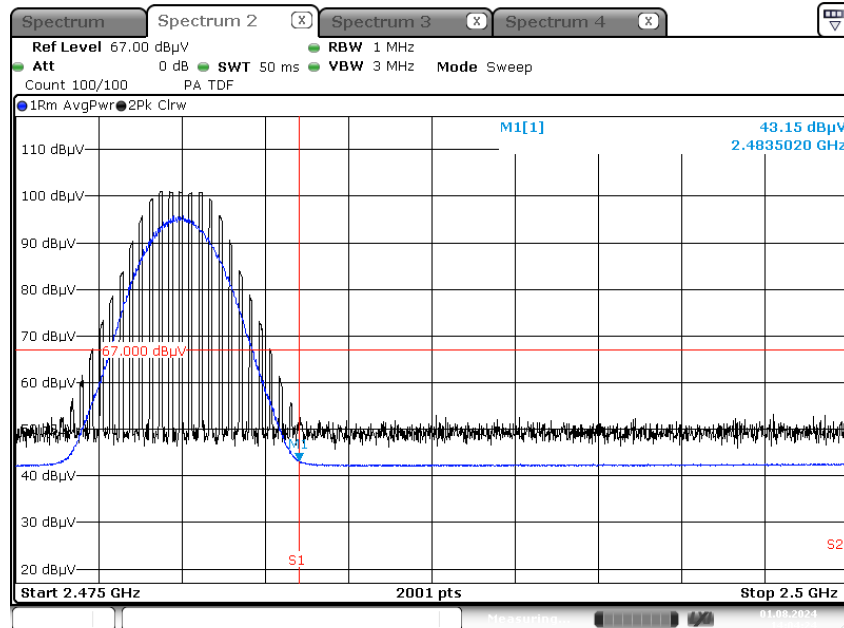
Radiated Restricted Band Edges plot – Average Result (Ch.39, Y-V)
