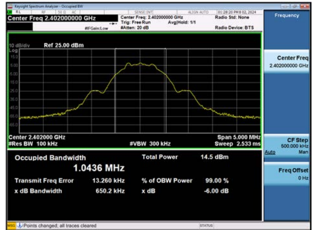
6 dB Bandwidth plot (Low-CH 0)
