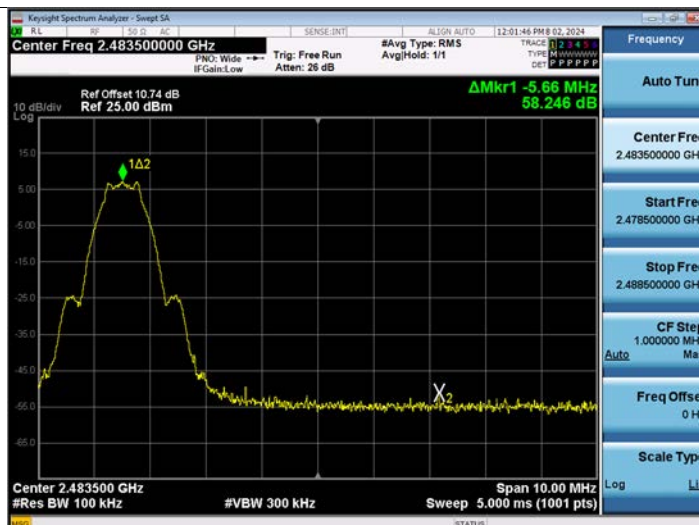
1M Bit/s (255 Byte) High-CH 39
