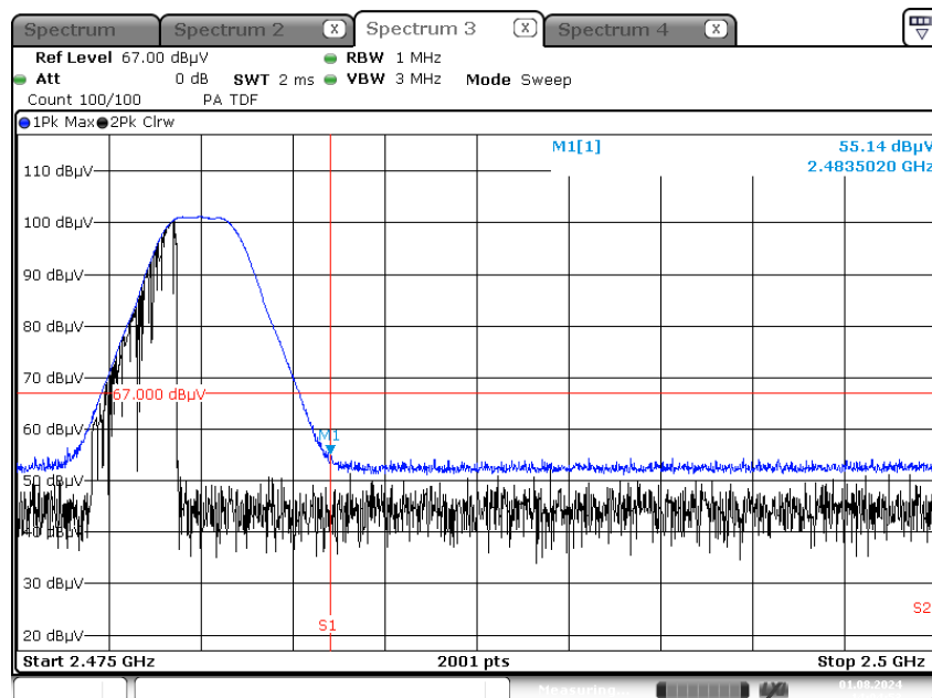
Radiated Restricted Band Edges plot – Peak Result (Ch.39, Y-V)
