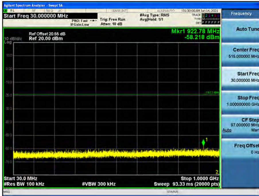
Conducted Spurious Emission (802.11n(20M)_Ch.1_MCS0)
