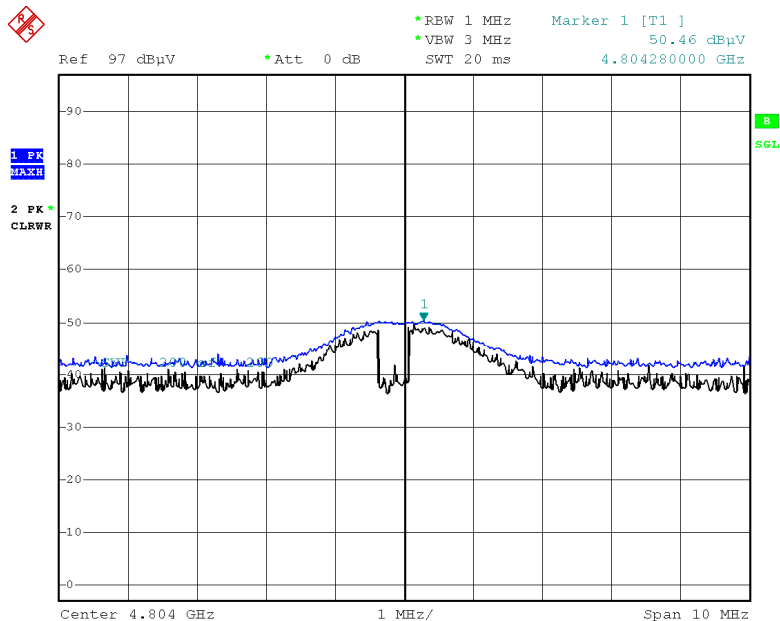
Radiated Spurious Emissions plot – Peak Reading (GFSK, Ch.0 2nd Harmonic, Y-V)
