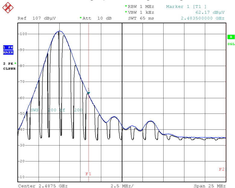
Radiated Restricted Band Edges plot – Average Reading (8DPSK, Ch.78, H)
