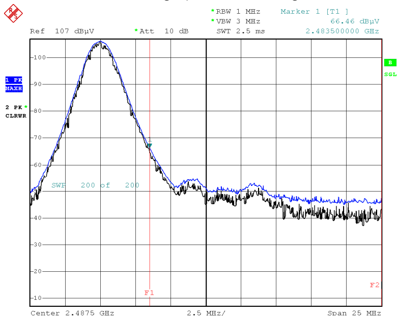
Radiated Restricted Band Edges plot –Peak Reading (8DPSK, Ch.78, H)
