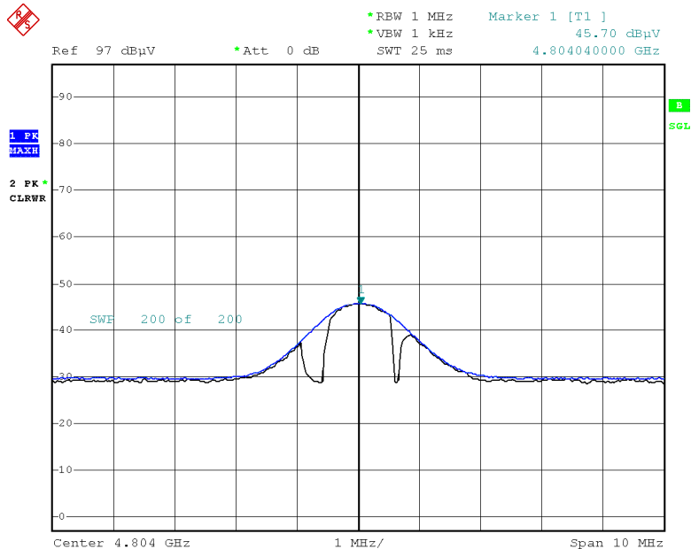
Radiated Spurious Emissions plot – Average Reading (GFSK, Ch.0 2nd Harmonic, Y-V)
