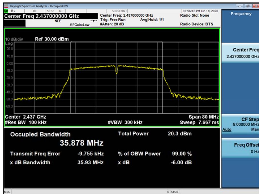
6dB Bandwidth plot (802.11n_HT40-CH 6)
