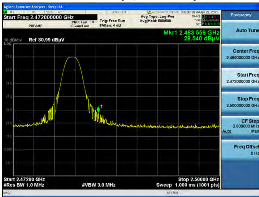
Radiated Restricted Band Edges plot – Peak Reading (Ch.39, Y-V)
