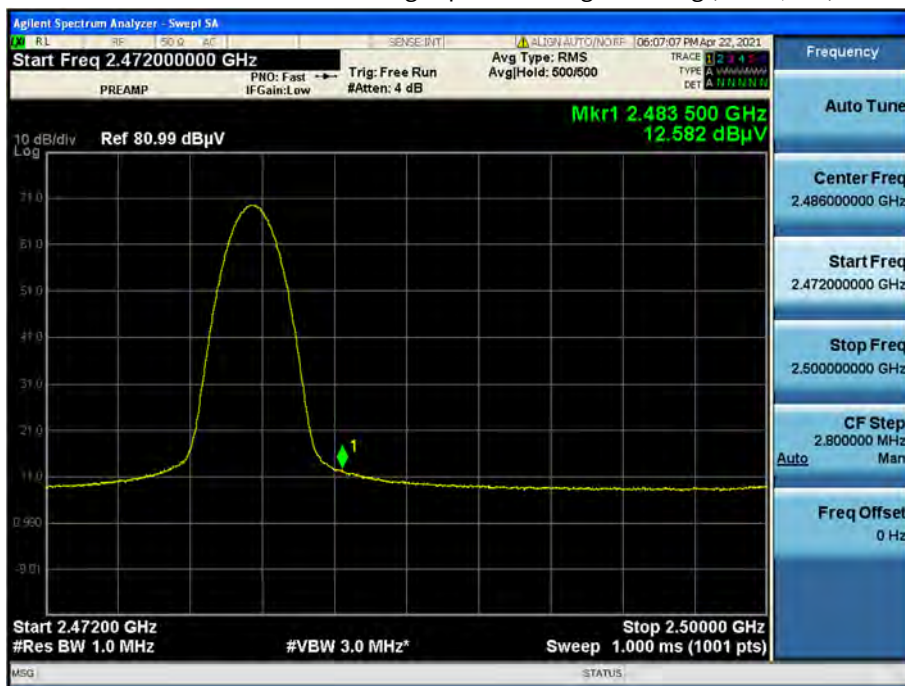
Radiated Restricted Band Edges plot – Average Reading (Ch.39, Y-V)
