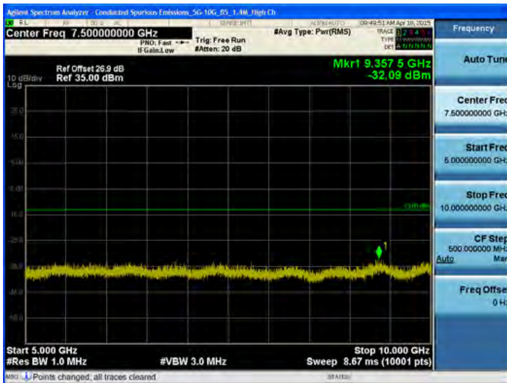
BAND 5. Conducted Spurious Plot _2 (20643ch_1.4MHz_QPSK_RB 1_0)
