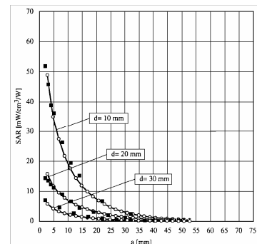
Figure 5-2 E-Field and temperature measurements at 1.9GHz [9]
