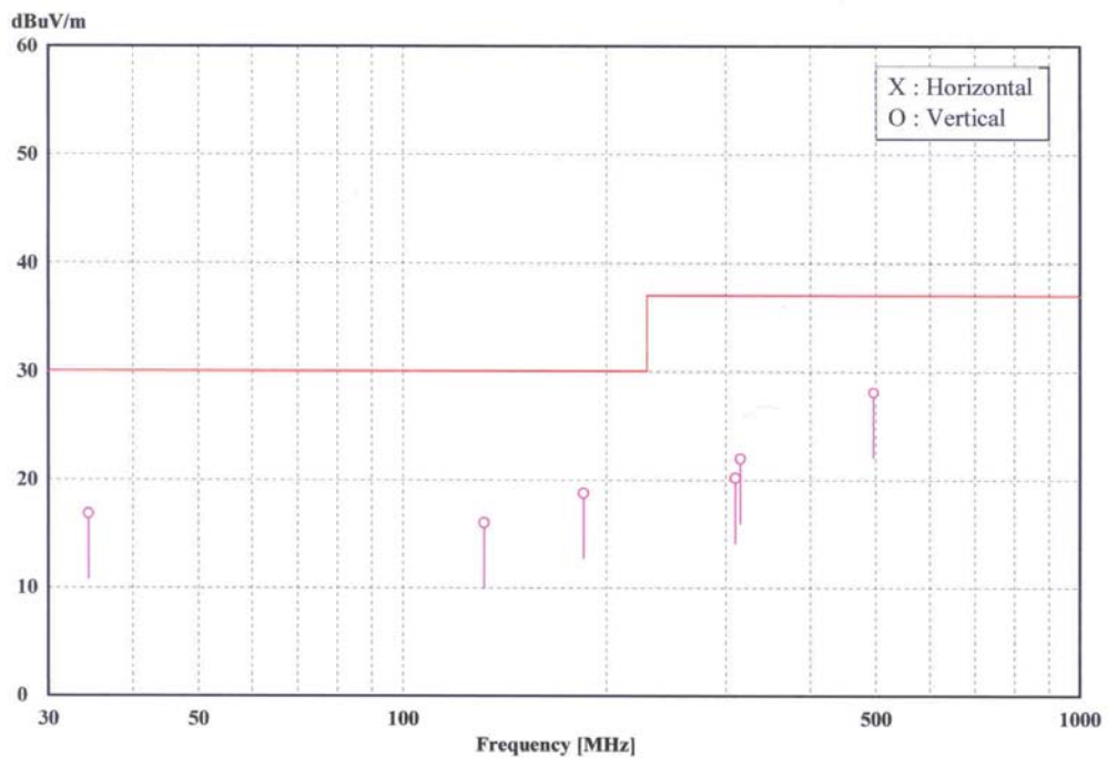
< Fig 6-2. Radiated emission result >
