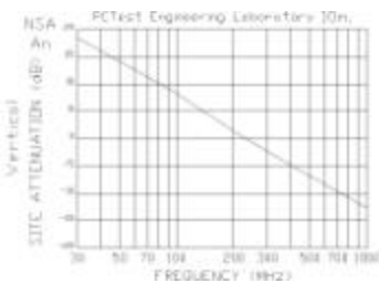
Fig. 6. NSA Theoretical Attenuation Curves (Vert. Pol.)
