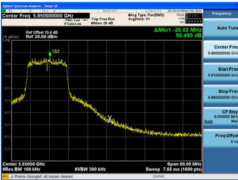
BandEdge (802.11a-CH 165)
