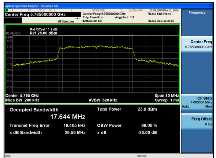
802.11n_20MHz UNII 3 BAND 99% Bandwidth(CH.153)
